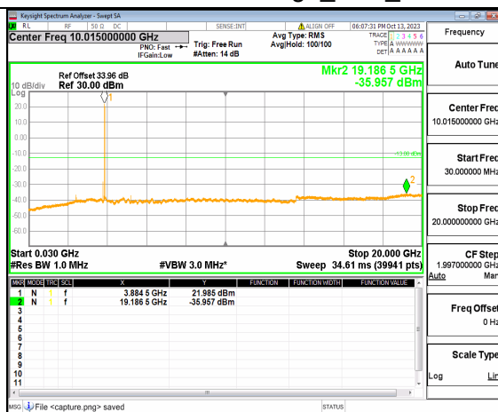
5A_n77(3700-3980MHz) (30MHz-20GHz) 90M DFT-s-OFDM BPSK Edge 1RB Right Mid
