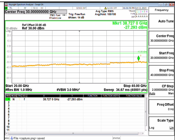
5A_n77(3700-3980MHz) (20GHz-40GHz) 90M DFT-s-OFDM BPSK Edge 1RB Left Mid
