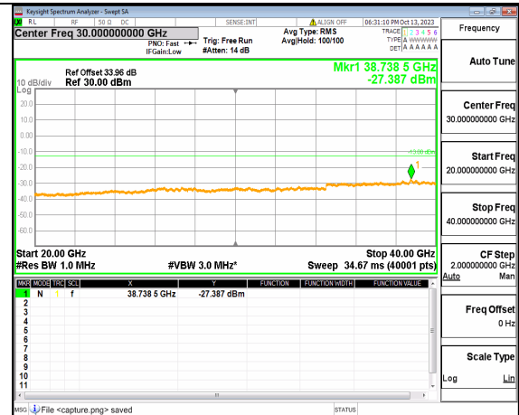
5A_n77(3700-3980MHz) (20GHz-40GHz) 100M DFT-s-OFDM BPSK Edge_1RB_Left Mid
