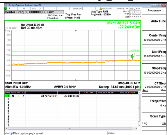
5A_n77(3700-3980MHz) (20GHz-40GHz) 90M DFT-s-OFDM BPSK Edge 1RB Right Mid
