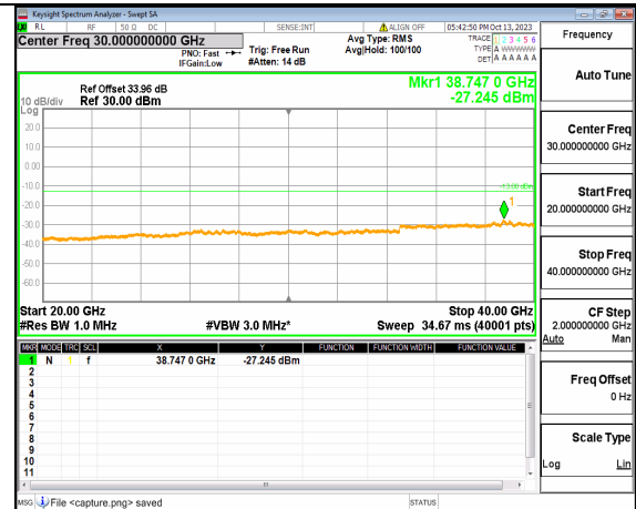
5A_n77(3700-3980MHz) (20GHz-40GHz) 80M DFT-s-OFDM BPSK Edge_1RB_Left Mid
