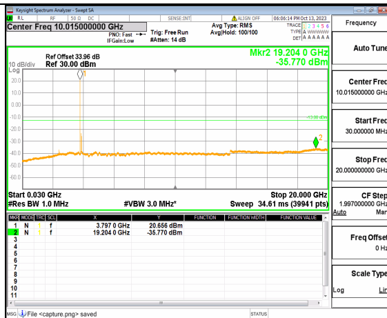
5A_n77(3700-3980MHz) (30MHz-20GHz) 90M DFT-s-OFDM BPSK Edge 1RB Left Mid
