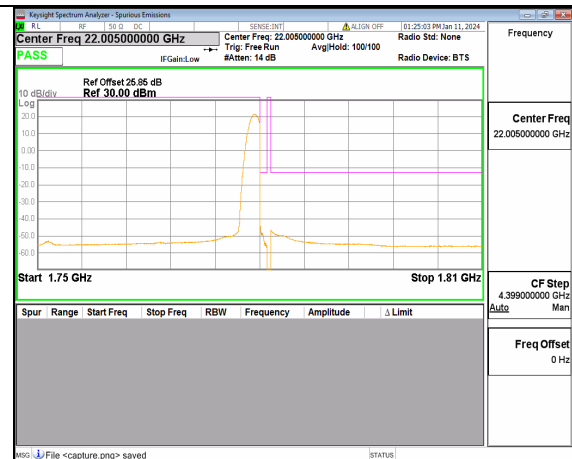
13A_n66 30M DFT-s-OFDM QPSK Edge_1RB_Right High
