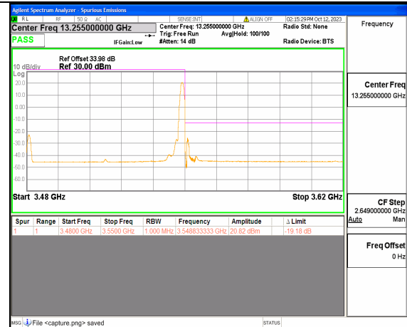
5A_n77(3450-3550MHz) 70M DFT-s-OFDM BPSK Edge_1RB_Right High
