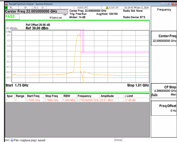
13A_n66 30M DFT-s-OFDM BPSK Edge_1RB_Right High
