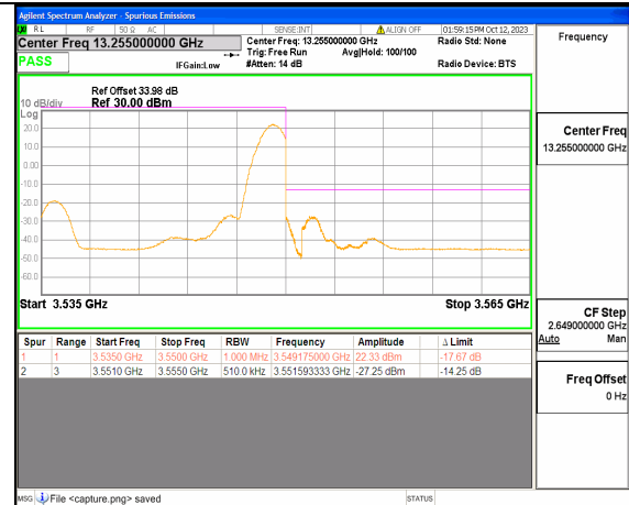
5A_n77(3450-3550MHz) 15M DFT-s-OFDM BPSK Edge_1RB_Right High
