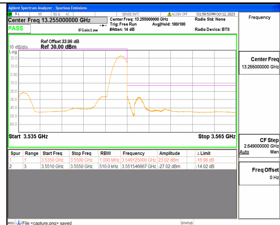
5A_n77(3450-3550MHz) 15M DFT-s-OFDM QPSK Edge_1RB_Right High
