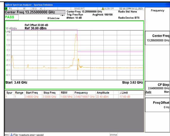
5A_n77(3450-3550MHz) 70M DFT-s-OFDM QPSK Edge_1RB_Right High
