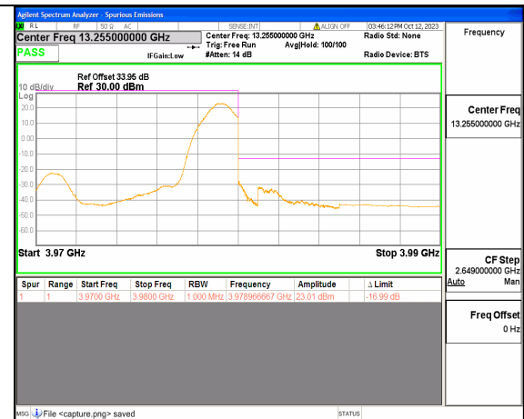
5A_n77(3700-3980MHz) 10M DFT-s-OFDM BPSK Edge_1RB_Right High
