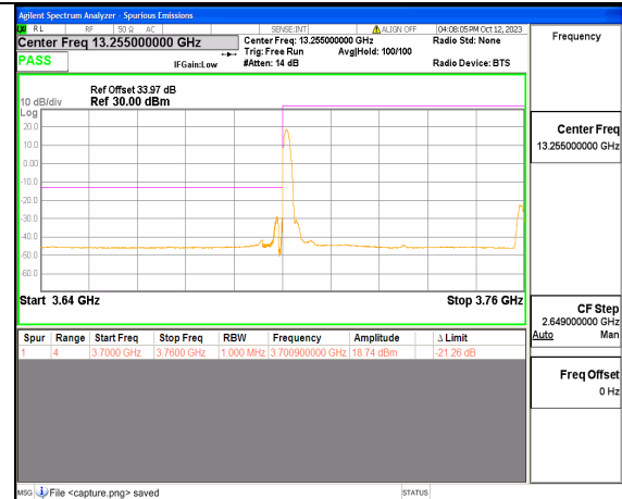
5A_n77(3700-3980MHz) 60M DFT-s-OFDM QPSK Edge_1RB_Left Low
