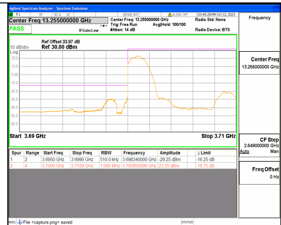
5A_n77(3700-3980MHz) 10M DFT-s-OFDM QPSK Edge_1RB_Left Low
