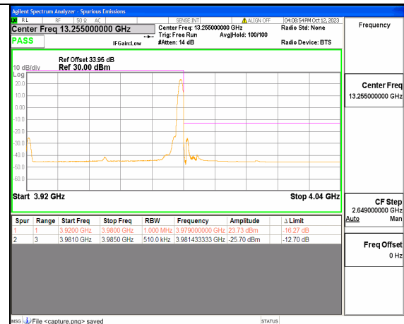
5A_n77(3700-3980MHz) 60M DFT-s-OFDM BPSK Edge_1RB_Right High
