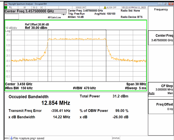
5A_n77(3450-3550MHz) 15M DFT-s-OFDM 64QAM Outer_Full Low
