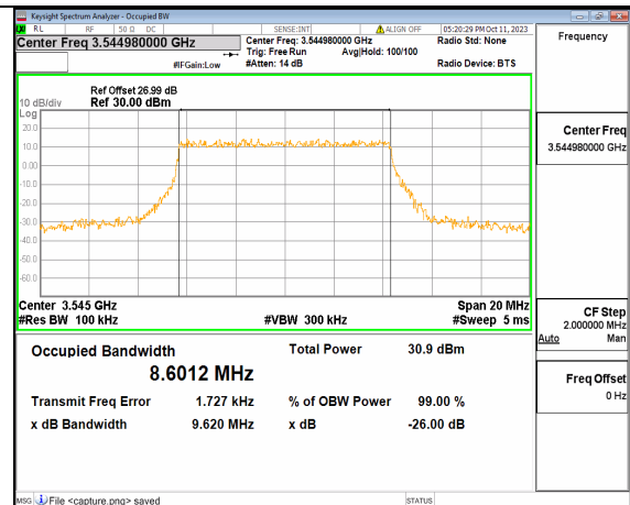
5A_n77(3450-3550MHz) 10M DFT-s-OFDM 64QAM Outer_Full High
