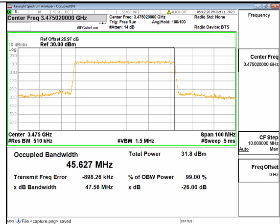
5A_n77(3450-3550MHz) 50M DFT-s-OFDM 64QAM Outer_Full Low
