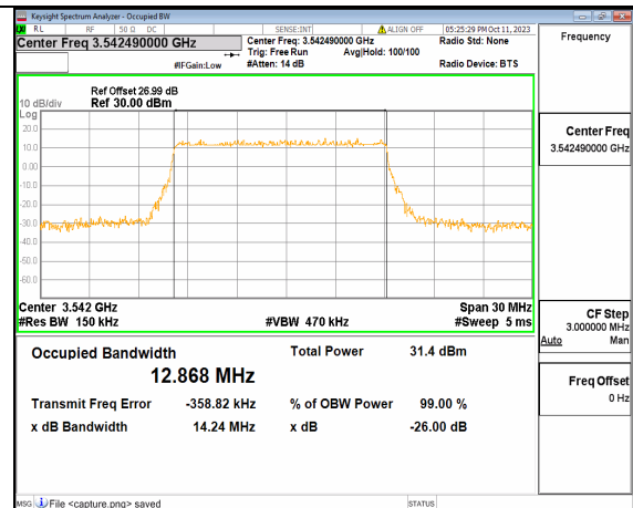
5A_n77(3450-3550MHz) 15M DFT-s-OFDM 64QAM Outer_Full High
