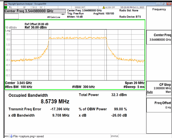
5A_n77(3450-3550MHz) 10M DFT-s-OFDM QPSK Outer_Full High
