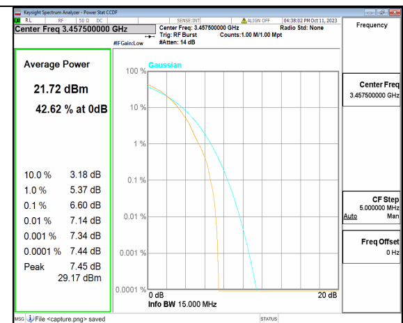
5A_n77(3450-3550MHz) 15M DFT-s-OFDM 256QAM Outer_Full Low
