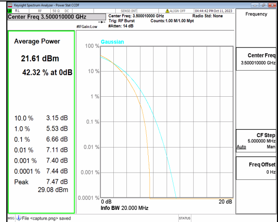
5A_n77(3450-3550MHz) 20M DFT-s-OFDM 256QAM Outer_Full Mid
