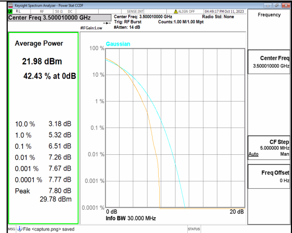
5A_n77(3450-3550MHz) 30M DFT-s-OFDM 256QAM Outer_Full Mid
