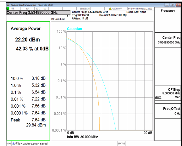
5A_n77(3450-3550MHz) 30M DFT-s-OFDM 256QAM Outer_Full High
