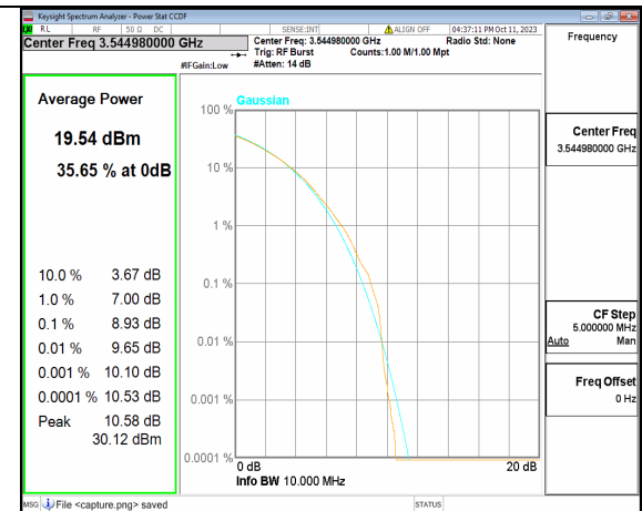
5A_n77(3450-3550MHz) 10M CP-OFDM 256QAM Outer_Full High
