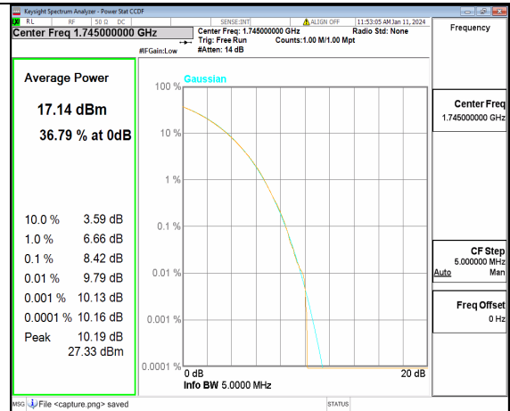
13A_n66 5M CP-OFDM 256QAM Outer_Full Mid
