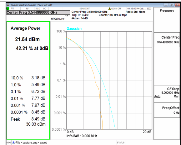
5A_n77(3450-3550MHz) 10M DFT-s-OFDM 256QAM Outer_Full High
