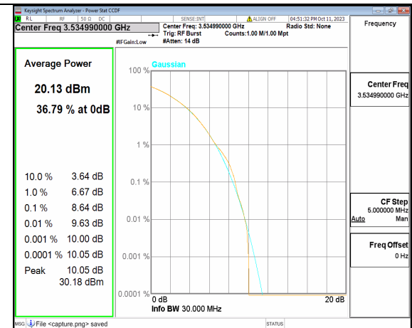
5A_n77(3450-3550MHz) 30M CP-OFDM 256QAM Outer_Full High
