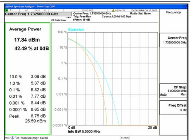
B4 / 5MHz / Mid CH / 256QAM
