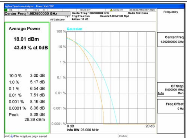
B2 / 15MHz / High CH / 256QAM
