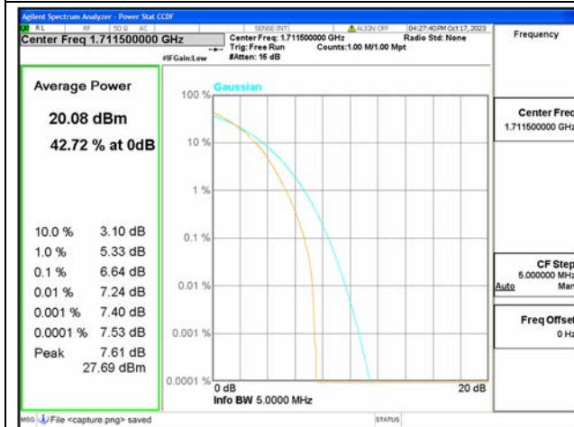
B4 / 3MHz / Low CH / 64QAM
