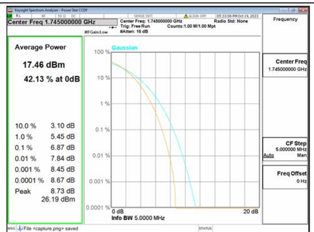
B66 / 3MHz / Mid CH / 256QAM
