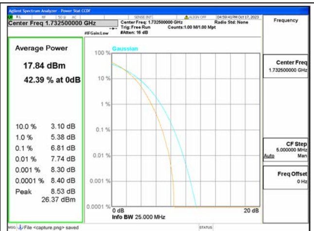
B4 / 15MHz / Mid CH / 256QAM
