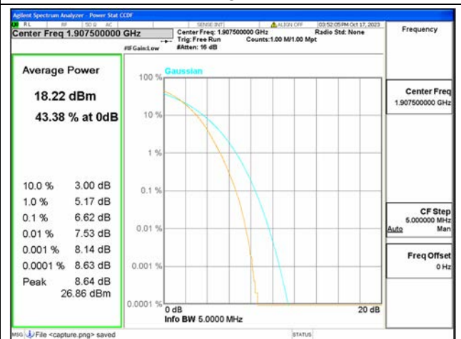
B2 / 5MHz / High CH / 256QAM
