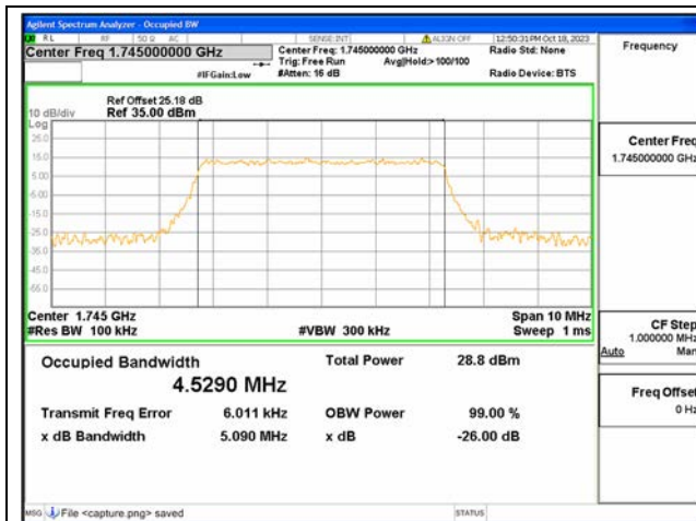
B66 / 5MHz / 64QAM/ Mid CH
