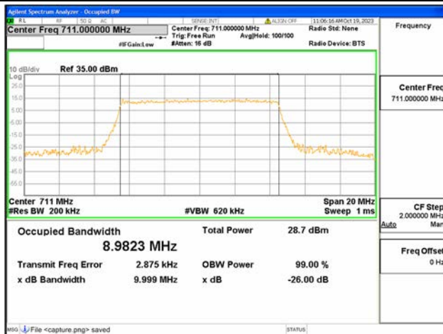
B12 / 10MHz / 64QAM/ High CH
