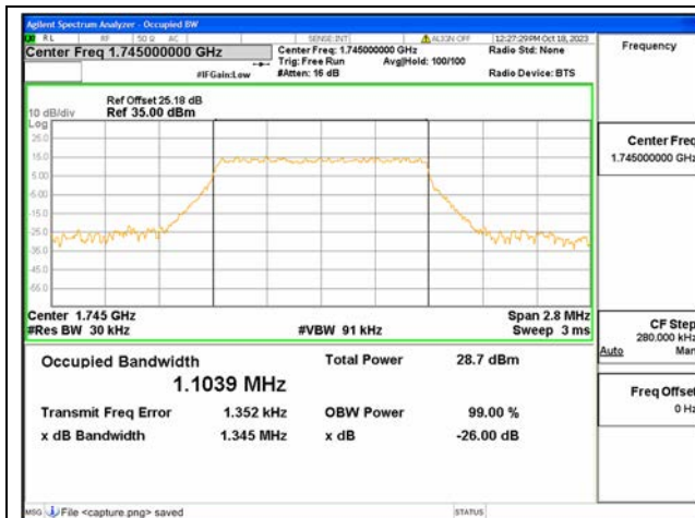
B66 / 1.4MHz / 64QAM/ Mid CH
