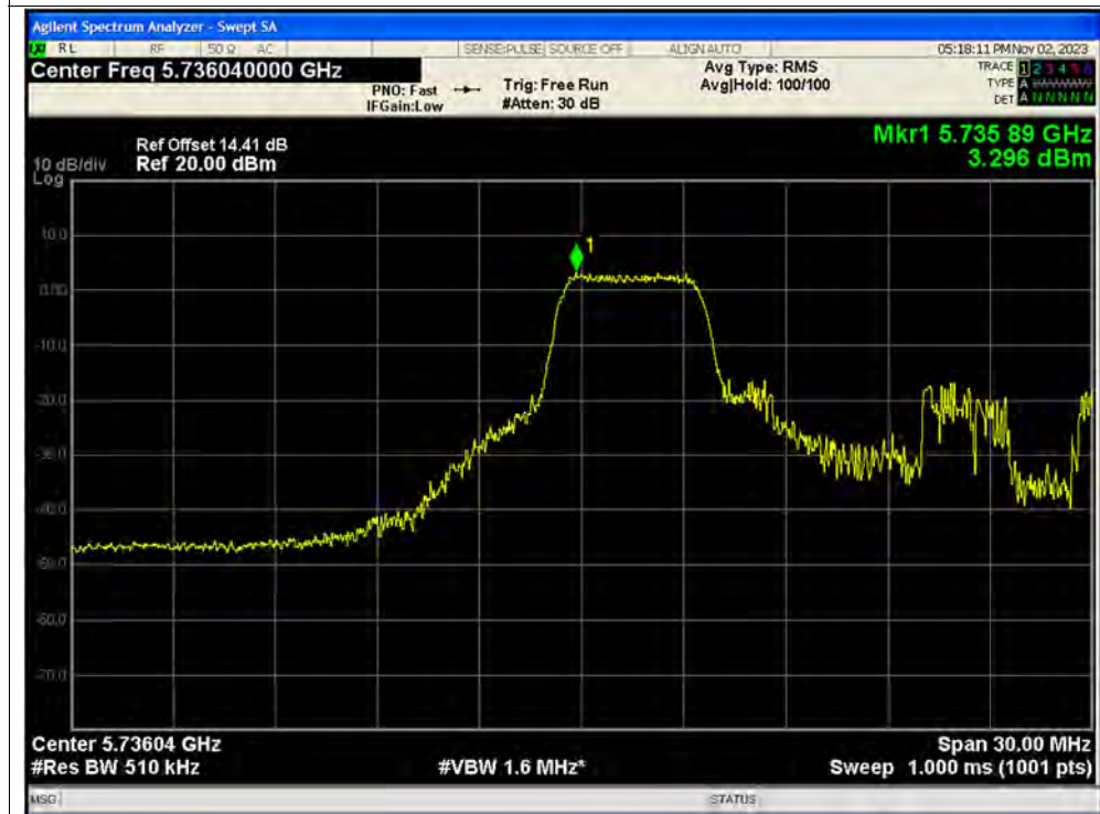
PSD NVNT ax20 52@37 5745MHz Ant2 MIMO
