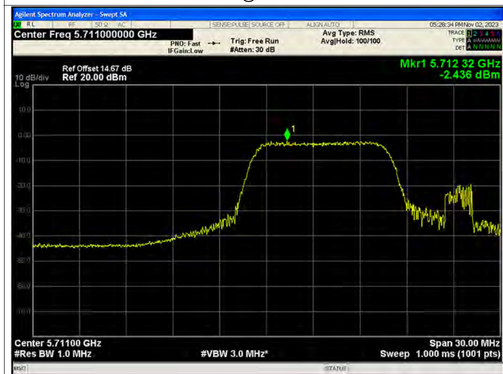
PSD NVNT ax20 106@53 5720MHz Ant2 MIMO
