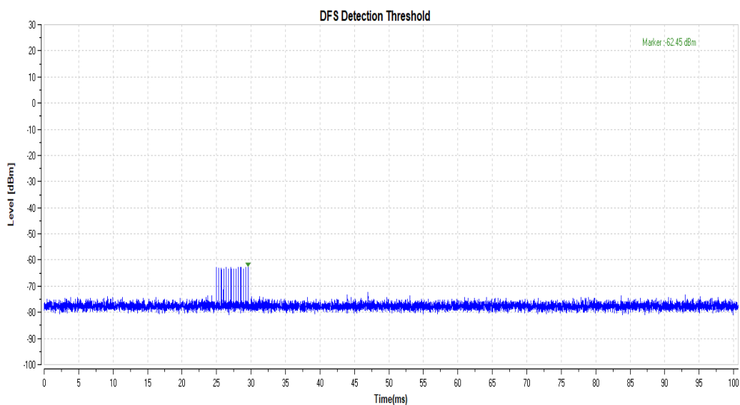
11AC160SISO_5570_Type5
