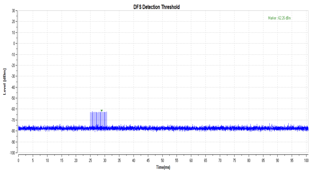
11AC160SISO_5570_Type4
