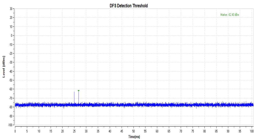
11AC160SISO_5570_Type6
