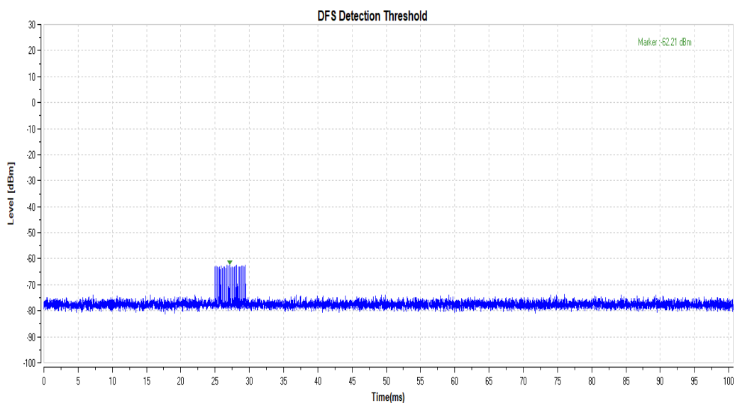
11AC160SISO_5570_Type3
