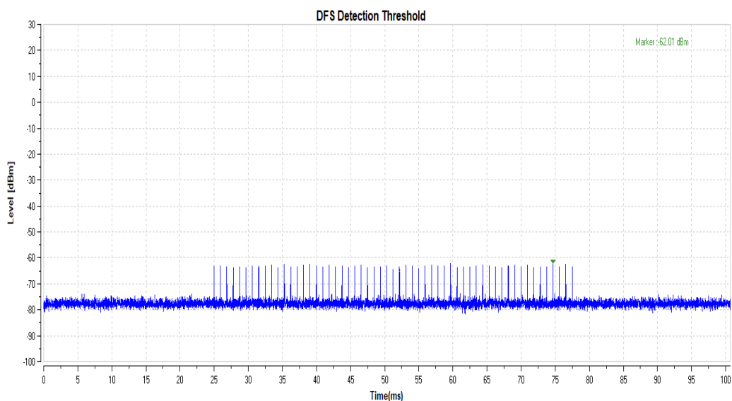
11AC160SISO_5570_Type2
