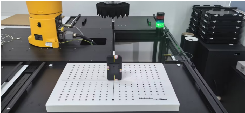
Right Side (Test distance: 2mm)
