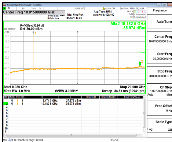
n77(3450-3550MHz) (30MHz-20GHz) 25M DFT-s-OFDM BPSK Inner_1RB_Right Low
