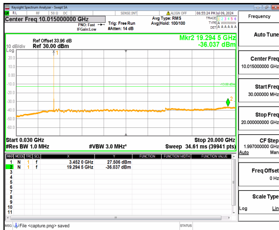
n77(3450-3550MHz) (30MHz-20GHz) 25M DFT-s-OFDM BPSK Inner_1RB_Left Low
