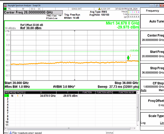
n77(3450-3550MHz) (20GHz-36GHz) 25M DFT-s-OFDM BPSK Inner_1RB_Right Mid
