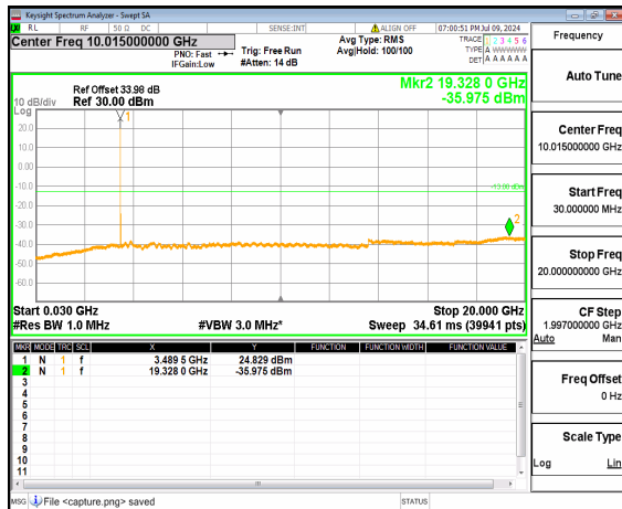
n77(3450-3550MHz) (30MHz-20GHz) 25M DFT-s-OFDM BPSK Inner_1RB_Left Mid
