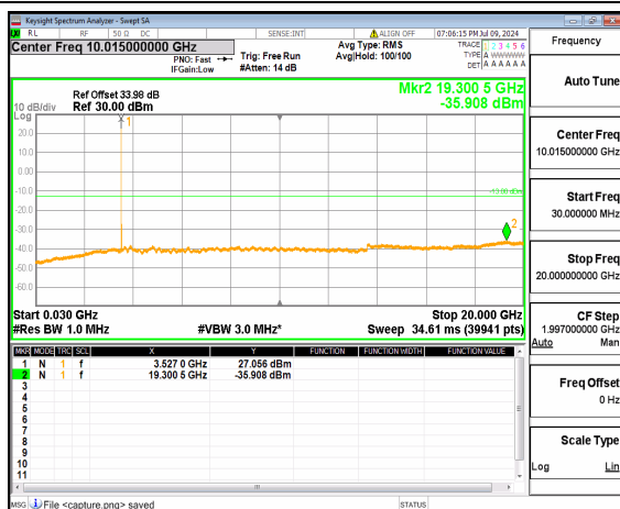
n77(3450-3550MHz) (30MHz-20GHz) 25M DFT-s-OFDM BPSK Inner_1RB_Left High
