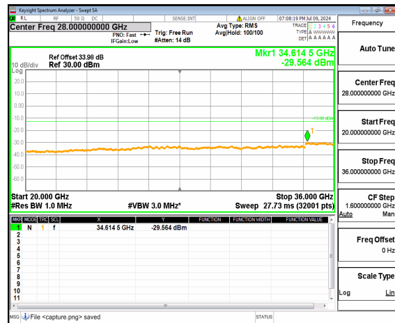
n77(3450-3550MHz) (20GHz-36GHz) 25M DFT-s-OFDM BPSK Inner_1RB_Right High
