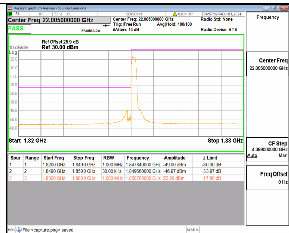
n2 30M DFT-s-OFDM BPSK Edge_1RB_Left Low
