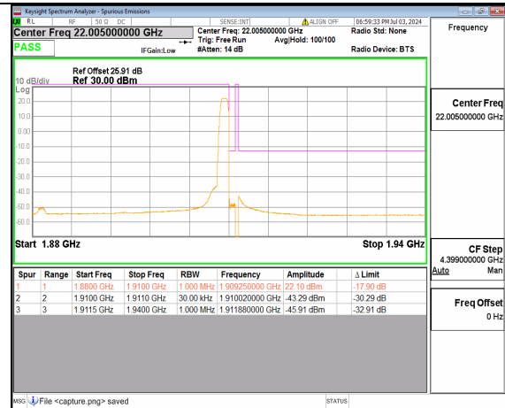
n2 30M DFT-s-OFDM BPSK Edge_1RB_Right High
