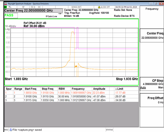
n2 25M DFT-s-OFDM BPSK Edge_1RB_Right High
