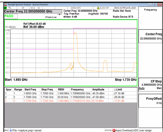
n66 25M DFT-s-OFDM BPSK Edge_1RB_Left Low
