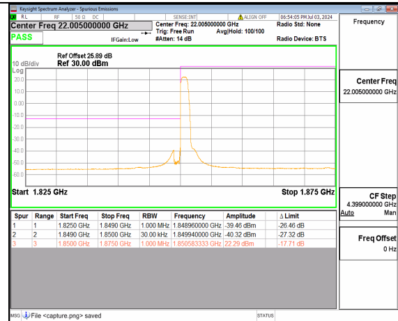
n2 25M DFT-s-OFDM BPSK Edge_1RB_Left Low
