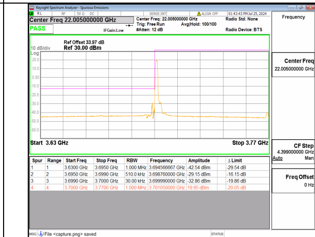
n78(3700-3800MHz) 70M DFT-s-OFDM BPSK Edge_1RB_Left Low
