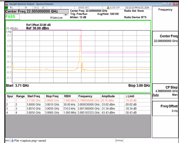
n78(3700-3800MHz) 90M DFT-s-OFDM QPSK Edge_1RB_Right High
