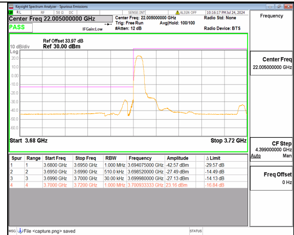
n78(3700-3800MHz) 20M DFT-s-OFDM BPSK Edge_1RB_Left Low
