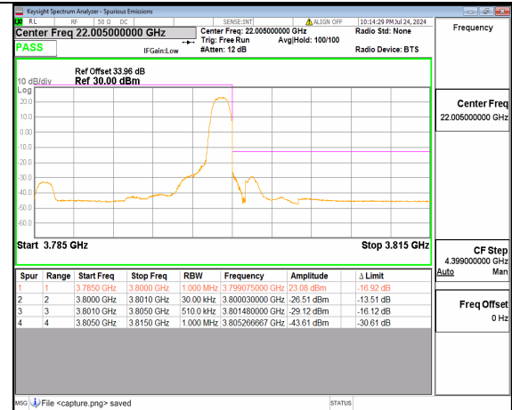
n78(3700-3800MHz) 15M DFT-s-OFDM QPSK Edge_1RB_Right High
