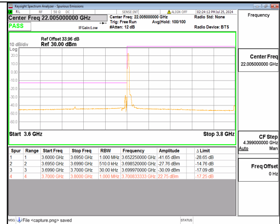
n78(3700-3800MHz) 100M DFT-s-OFDM BPSK Edge_1RB_Left Low
