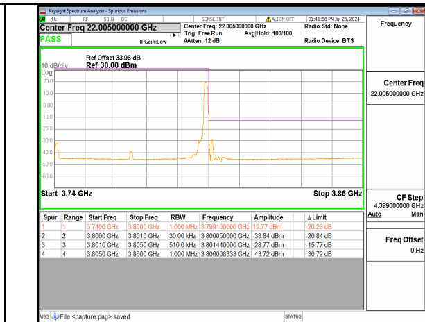
n78(3700-3800MHz) 60M DFT-s-OFDM QPSK Edge_1RB_Right High
