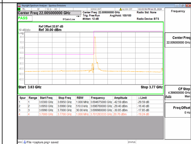
n78(3700-3800MHz) 70M DFT-s-OFDM QPSK Edge_1RB_Left Low
