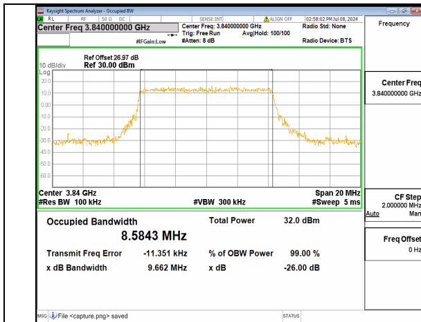
n77(3700-3980MHz) 10M DFT-s-OFDM BPSK Outer_Full Mid
