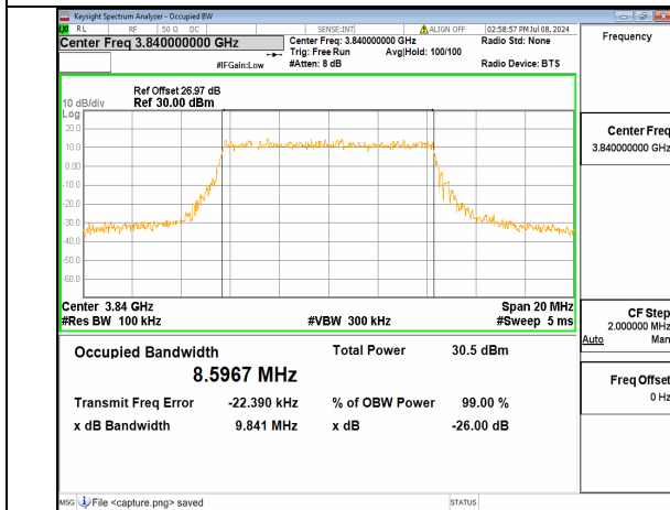
n77(3700-3980MHz) 10M DFT-s-OFDM 16QAM Outer_Full Mid
