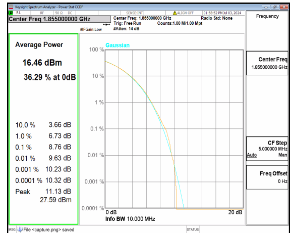
n2 10M CP-OFDM 256QAM Outer_Full Low
