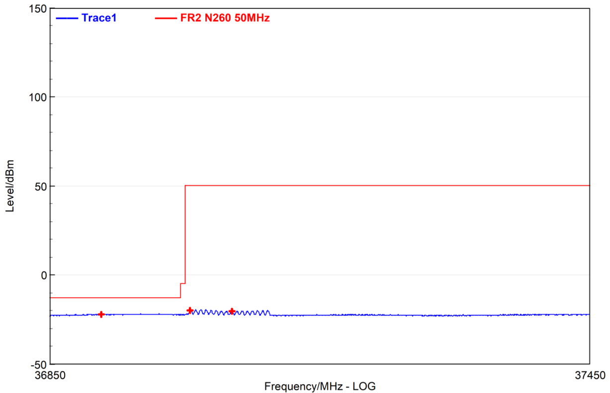
n260 Module 0 SCS 120kHz Full RB Beam ID 13+269 PUSCH DFT 100M Low Y V
