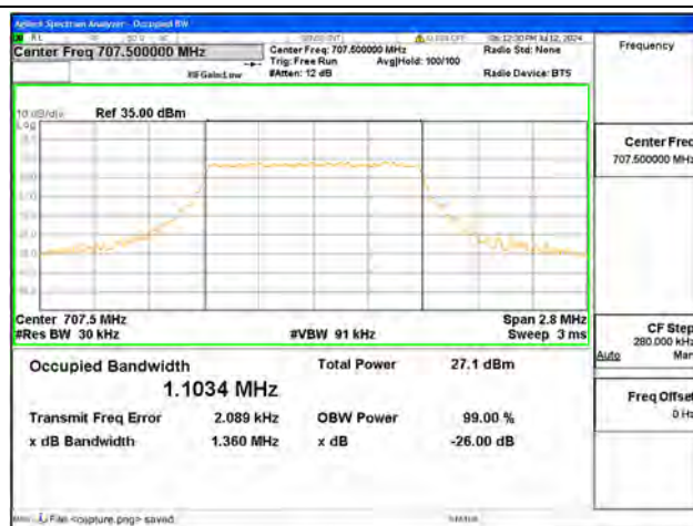
B12 / 1.4MHz / 64QAM/ Mid CH
