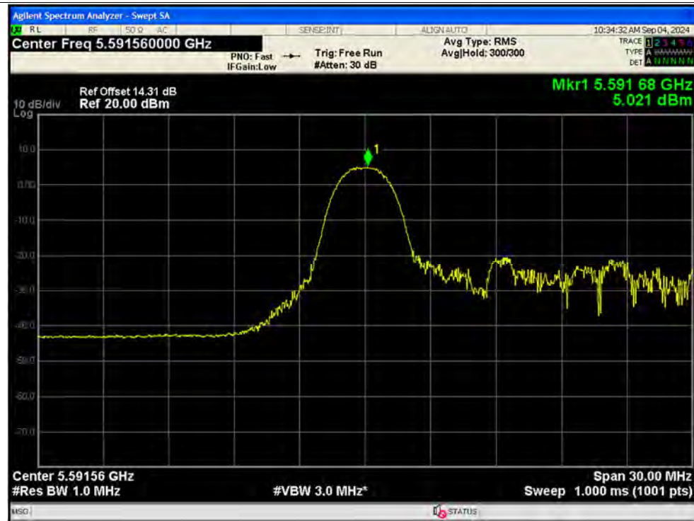
PSD NVNT ax20 26@0 5600MHz Ant2 MIMO
