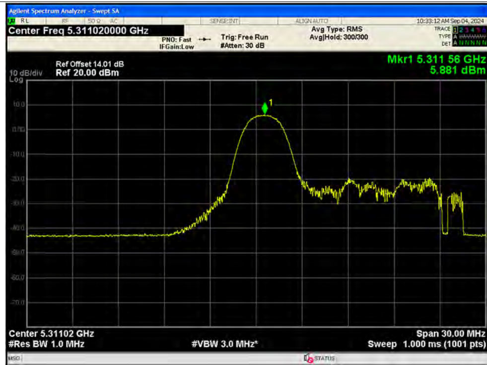
PSD NVNT ax20 26@0 5320MHz Ant2 MIMO
