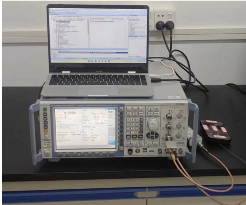
Test setup
