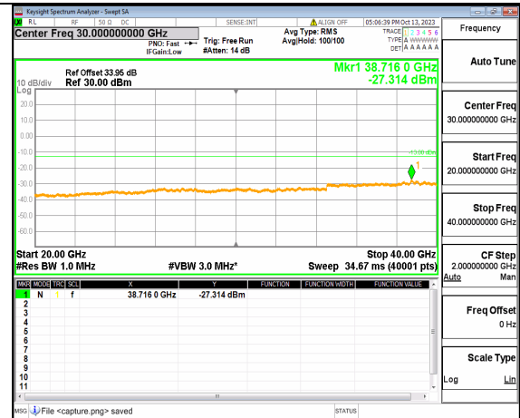
5A_n77(3700-3980MHz) (20GHz-40GHz) 60M DFT-s-OFDM QPSK Edge_1RB_Left High
