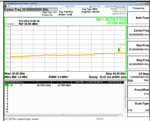
5A_n77(3700-3980MHz) (20GHz-40GHz) 60M DFT-s-OFDM BPSK Edge_1RB_Left Mid
