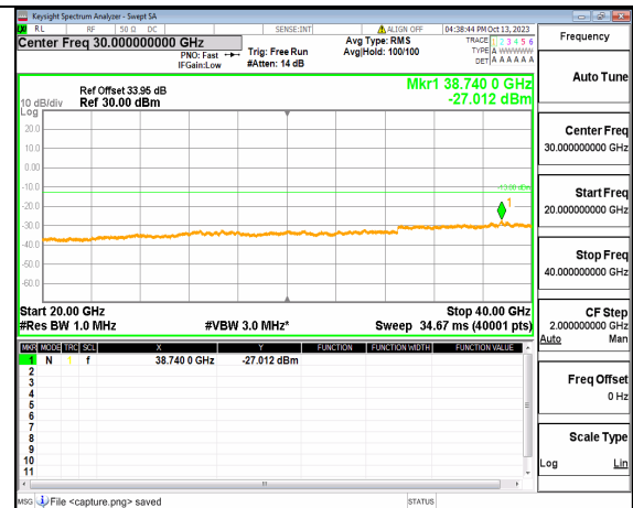
5A_n77(3700-3980MHz) (20GHz-40GHz) 50M DFT-s-OFDM BPSK Edge_1RB_Left High
