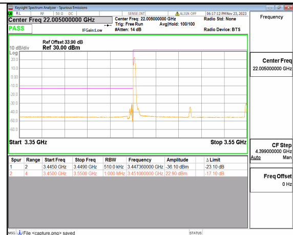
5A_n77 (3450-3550MHz) 100M DFT-s-OFDM BPSK Edge_1RB_Left Low
