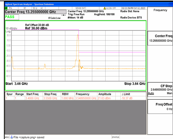
5A_n77(3450-3550MHz) 90M DFT-s-OFDM QPSK Edge_1RB_Right High
