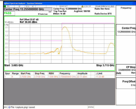
5A_n77(3700-3980MHz) 15M DFT-s-OFDM BPSK Edge_1RB_Left Low
