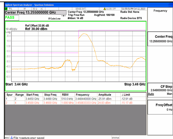
5A_n77(3450-3550MHz) 10M DFT-s-OFDM QPSK Edge_1RB_Left Low
