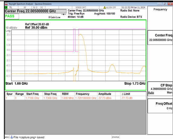
13A_n66 20M DFT-s-OFDM BPSK Edge_1RB_Left Low
