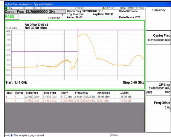
5A_n77(3450-3550MHz) 10M DFT-s-OFDM BPSK Edge_1RB_Left Low
