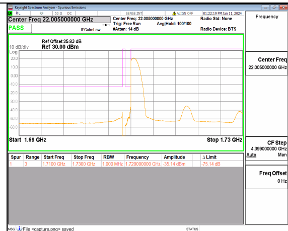
13A_n66 20M DFT-s-OFDM QPSK Edge_1RB_Left Low
