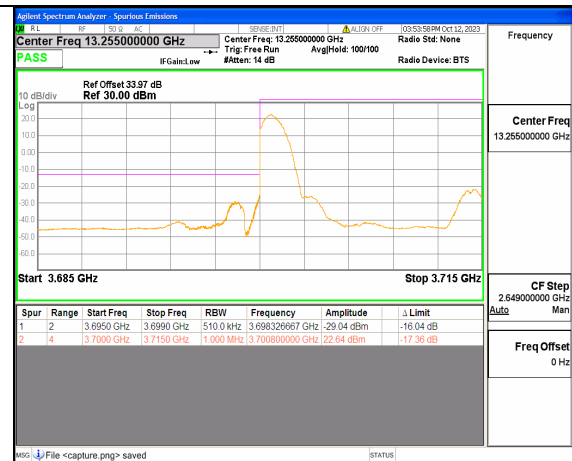
5A_n77(3700-3980MHz) 15M DFT-s-OFDM QPSK Edge_1RB_Left Low
