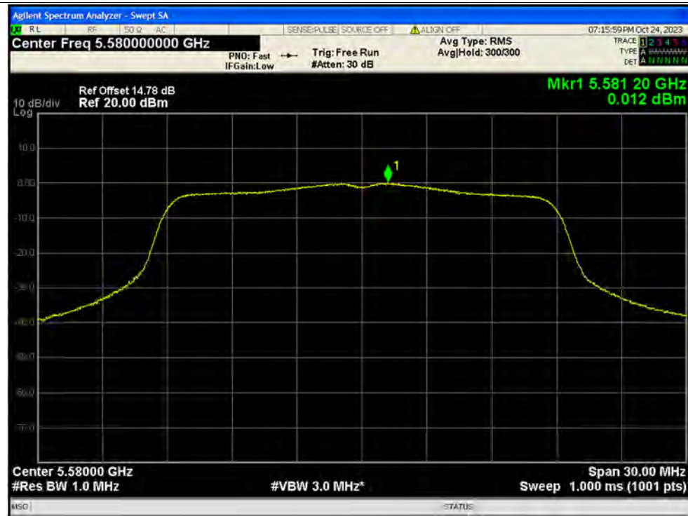
PSD NVNT n20 5580MHz Ant2 MIMO
