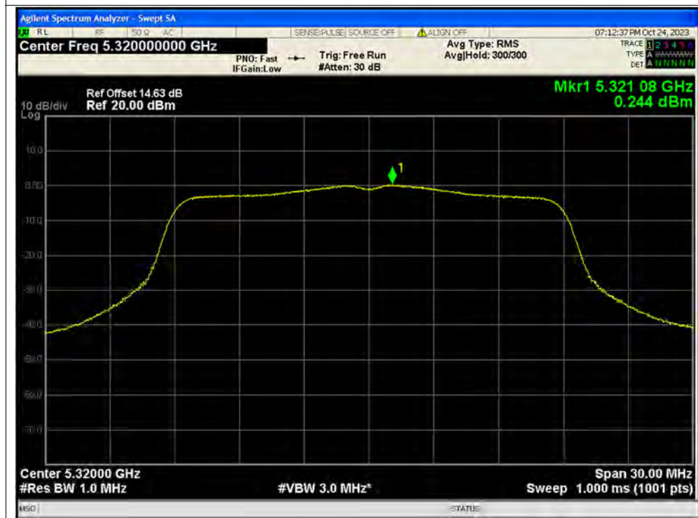
PSD NVNT n20 5320MHz Ant2 MIMO
