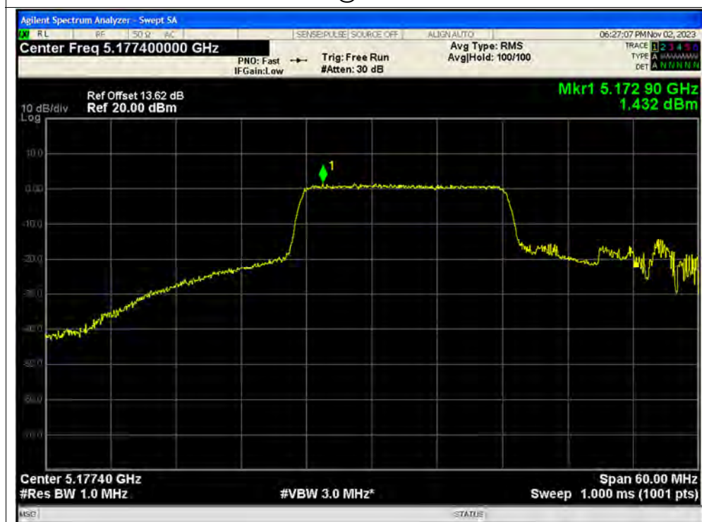
PSD NVNT ax40 242@61 5190MHz Ant2 MIMO
