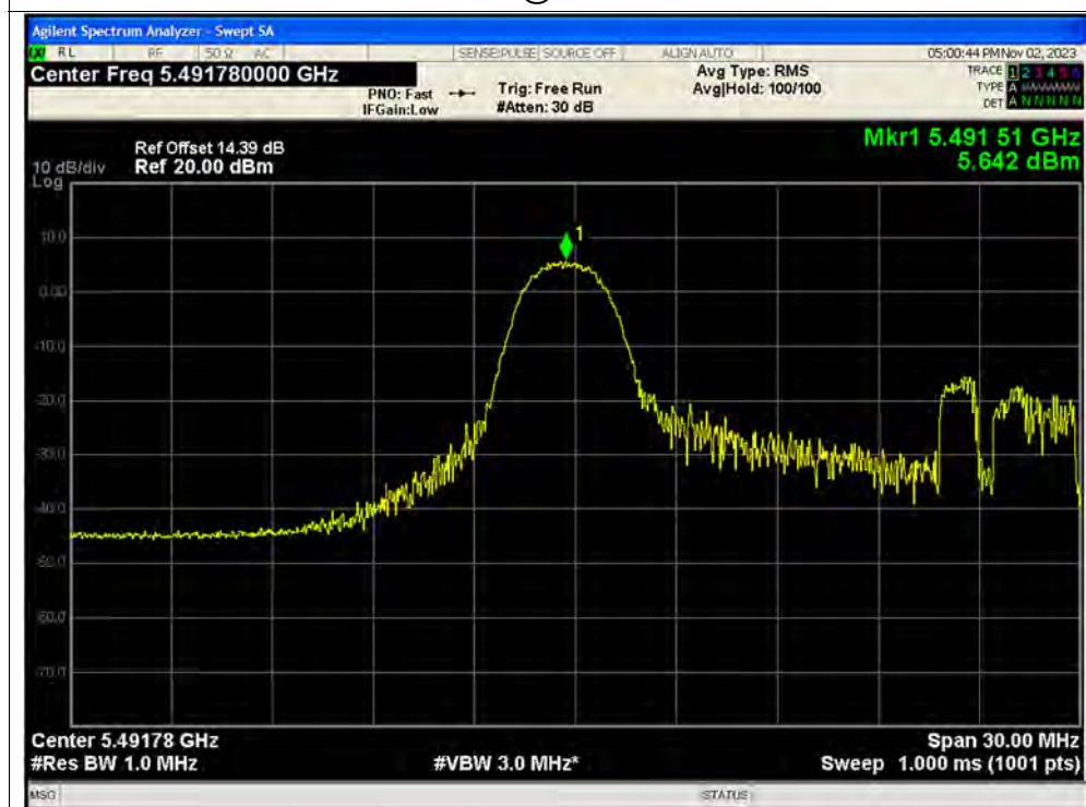
PSD NVNT ax20 26@0 5500MHz Ant2 MIMO
