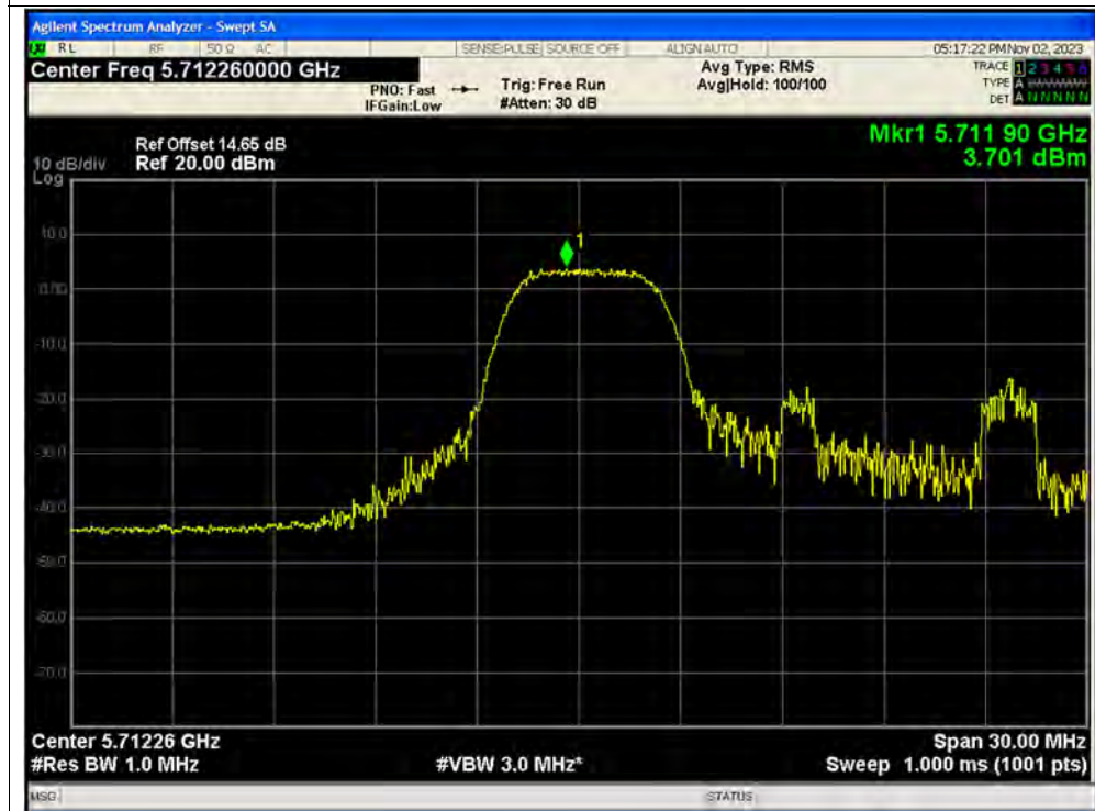
PSD NVNT ax20 52@37 5720MHz Ant2 MIMO
