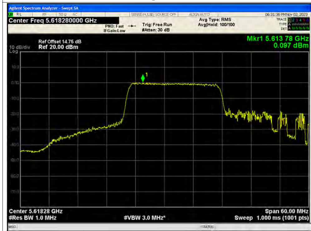
PSD NVNT ax40 242@61 5630MHz Ant2 MIMO
