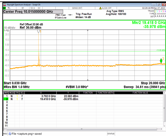
2A_n77(3700-3980MHz) (30MHz-20GHz) 100M DFT-s-OFDM BPSK Inner_1RB_Left Low
