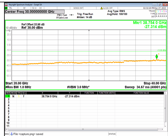
2A_n77(3700-3980MHz) (20GHz-40GHz) 100M DFT-s-OFDM QPSK Inner_1RB_Left Low
