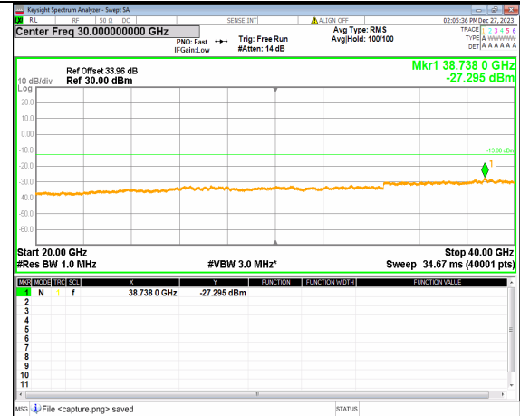
2A_n77(3700-3980MHz) (20GHz-40GHz) 60M DFT-s-OFDM BPSK Inner_1RB_Left Mid
