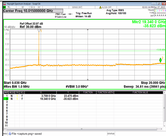
2A_n77(3700-3980MHz) (30MHz-20GHz) 60M DFT-s-OFDM BPSK Inner_1RB_Right Low
