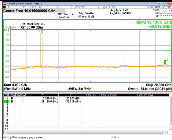
2A_n77(3700-3980MHz) (30MHz-20GHz) 100M DFT-s-OFDM BPSK Inner_1RB_Right Low
