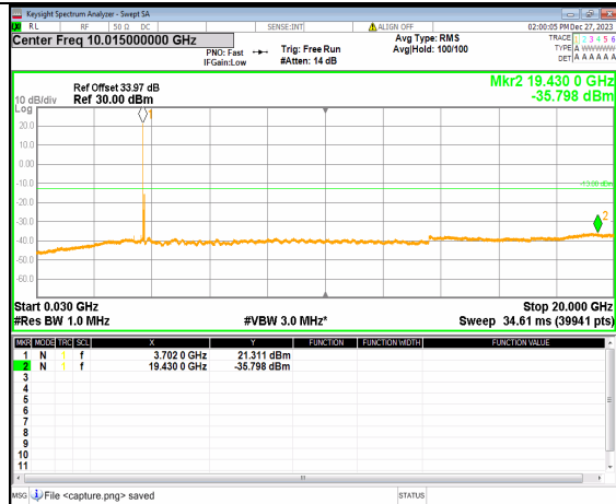
2A_n77(3700-3980MHz) (30MHz-20GHz) 60M DFT-s-OFDM BPSK Inner_1RB_Left Low
