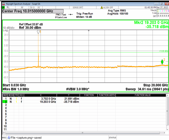
2A_n77(3700-3980MHz) (30MHz-20GHz) 40M DFT-s-OFDM BPSK Inner_1RB_Left Low
