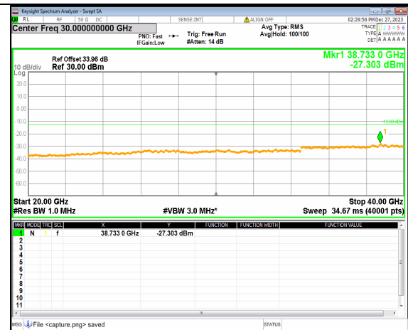
2A_n77(3700-3980MHz) (20GHz-40GHz) 100M DFT-s-OFDM BPSK Inner_1RB_Left Low
