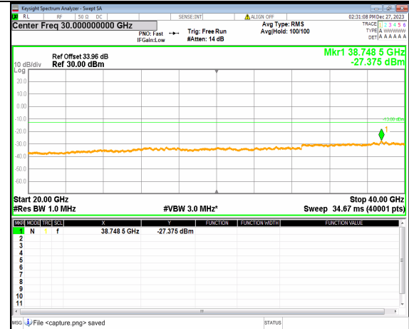
2A_n77(3700-3980MHz) (20GHz-40GHz) 100M DFT-s-OFDM BPSK Inner_1RB_Right Low
