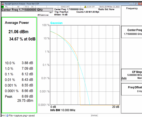
2A_n66 10M CP-OFDM QPSK Outer_Full Low
