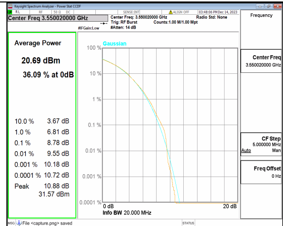
2A_n77(3450-3650MHz) 20M CP-OFDM 256QAM Outer_Full Mid
