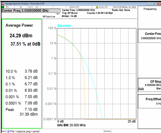
2A_n77(3450-3650MHz) 20M CP-OFDM QPSK Outer_Full Mid
