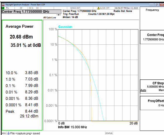
2A_n66 15M CP-OFDM QPSK Outer_Full High
