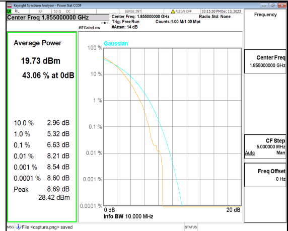
5A_n2 10M DFT-s-OFDM 256QAM Outer_Full Low
