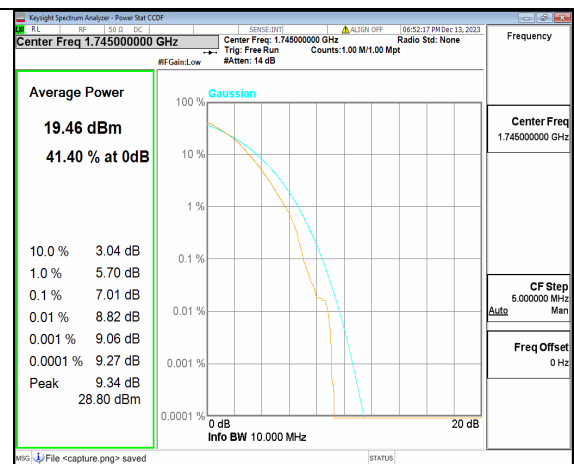
2A_n66 10M DFT-s-OFDM 256QAM Outer_Full Mid
