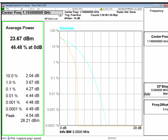
2A_n66 5M DFT-s-OFDM BPSK Outer_Full Mid
