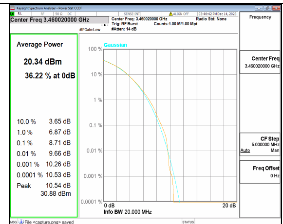
2A_n77(3450-3650MHz) 20M CP-OFDM 256QAM Outer_Full Low
