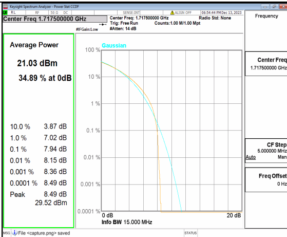
2A_n66 15M CP-OFDM QPSK Outer_Full Low
