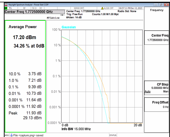
2A_n66 15M CP-OFDM 256QAM Outer_Full High
