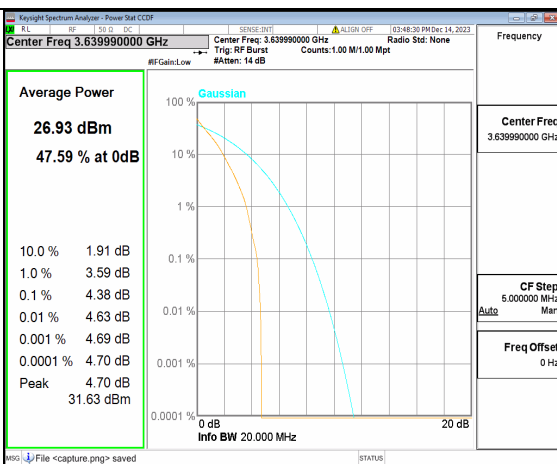
2A_n77(3450-3650MHz) 20M DFT-s-OFDM BPSK Outer_Full High
