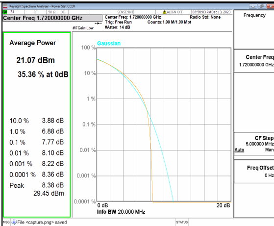
2A_n66 20M CP-OFDM QPSK Outer_Full Low
