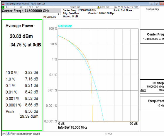
2A_n66 15M CP-OFDM QPSK Outer_Full Mid
