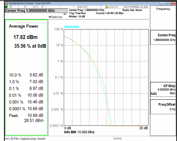
5A_n2 10M CP-OFDM 256QAM Outer_Full Mid
