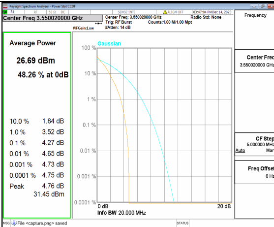
2A_n77(3450-3650MHz) 20M DFT-s-OFDM BPSK Outer_Full Mid
