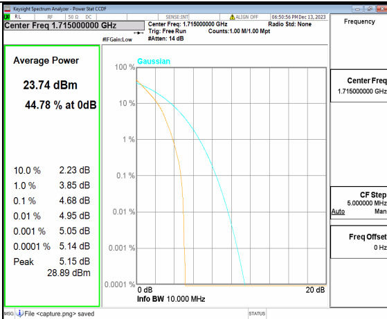
2A_n66 10M DFT-s-OFDM BPSK Outer_Full Low
