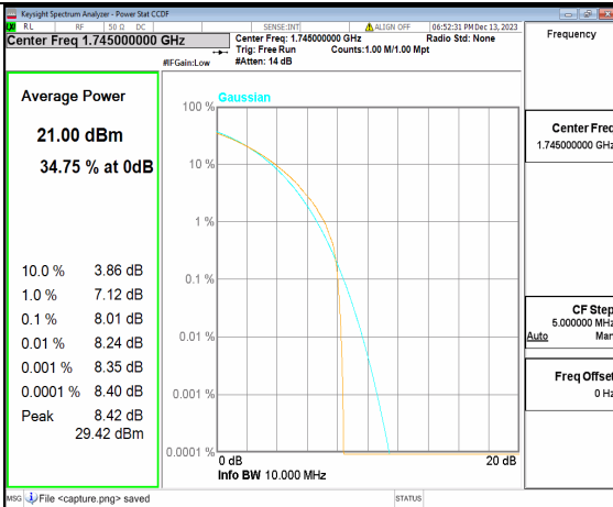
2A_n66 10M CP-OFDM QPSK Outer_Full Mid
