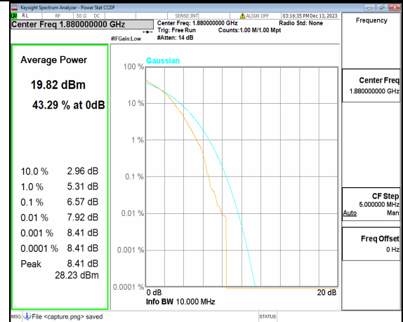
5A_n2 10M DFT-s-OFDM 256QAM Outer_Full Mid
