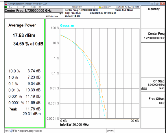
2A_n66 20M CP-OFDM 256QAM Outer_Full Low
