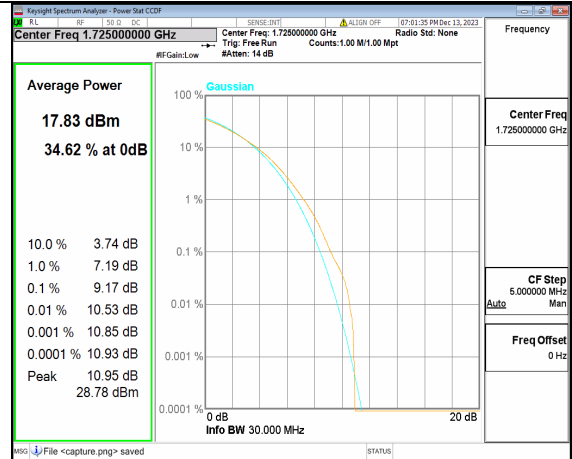
2A_n66 30M CP-OFDM 256QAM Outer_Full Low
