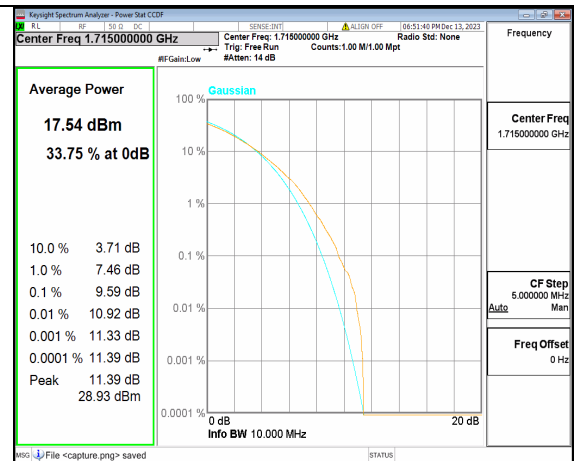
2A_n66 10M CP-OFDM 256QAM Outer_Full Low
