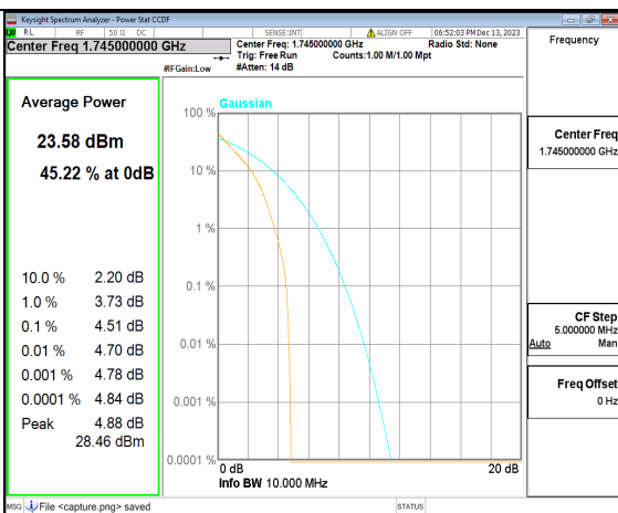
2A_n66 10M DFT-s-OFDM BPSK Outer_Full Mid
