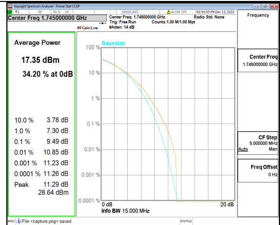
2A_n66 15M CP-OFDM 256QAM Outer_Full Mid
