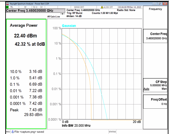
2A_n77(3450-3650MHz) 20M DFT-s-OFDM 256QAM Outer_Full Low
