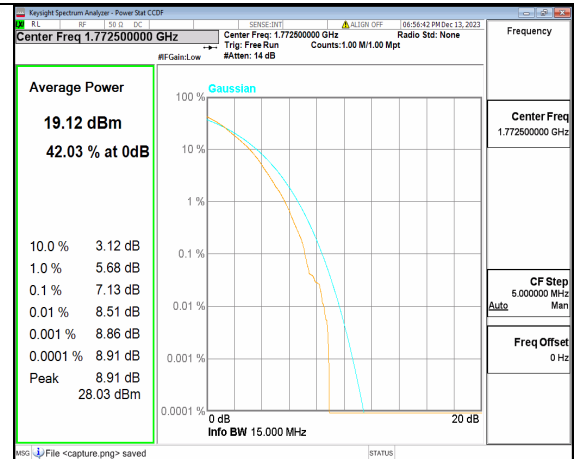
2A_n66 15M DFT-s-OFDM 256QAM Outer_Full High
