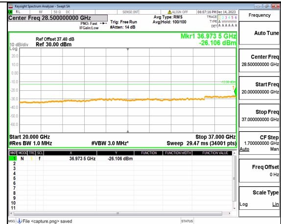
2A_n77(3450-3650MHz) (20GHz-37GHz) 100M DFT-s-OFDM QPSK Inner_1RB_Right Mid
