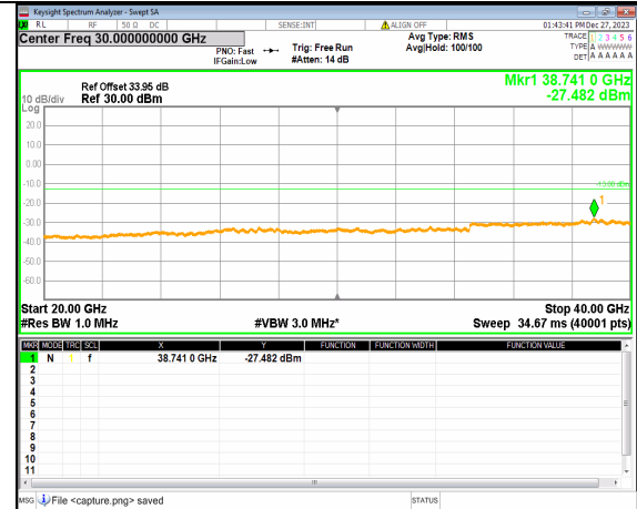
2A_n77(3700-3980MHz) (20GHz-40GHz) 30M DFT-s-OFDM QPSK Inner_1RB_Left High
