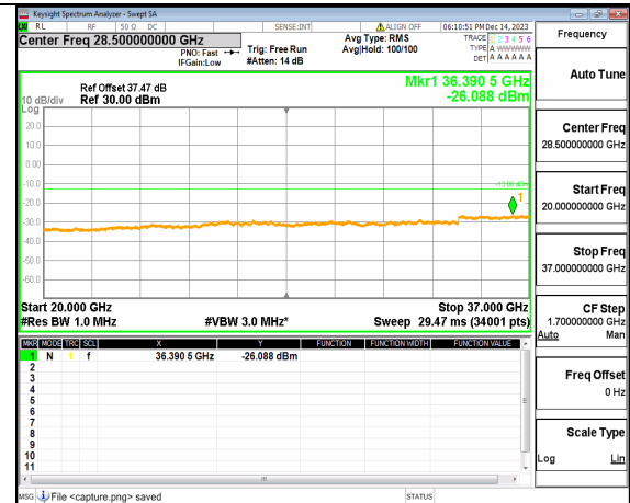
2A_n77(3450-3650MHz) (20GHz-37GHz) 100M DFT-s-OFDM QPSK Inner_1RB_Left High
