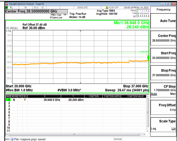
2A_n77(3450-3650MHz) (20GHz-37GHz) 100M DFT-s-OFDM BPSK Inner_1RB_Right Low
