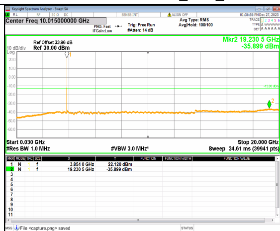
2A_n77(3700-3980MHz) (30MHz-20GHz) 30M DFT-s-OFDM BPSK Inner_1RB_Right Mid
