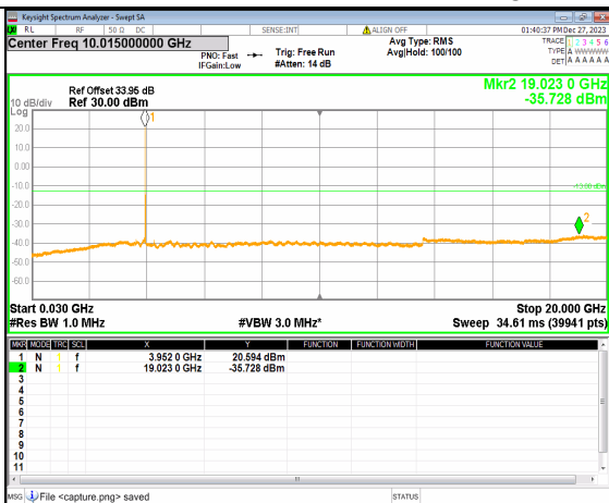
2A_n77(3700-3980MHz) (30MHz-20GHz) 30M DFT-s-OFDM BPSK Inner_1RB_Left High
