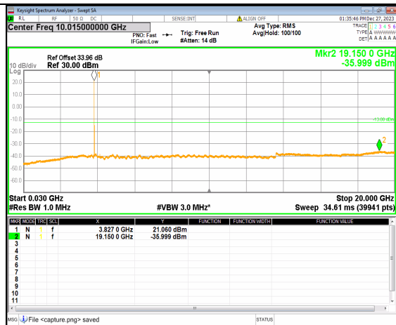
2A_n77(3700-3980MHz) (30MHz-20GHz) 30M DFT-s-OFDM BPSK Inner_1RB_Left Mid
