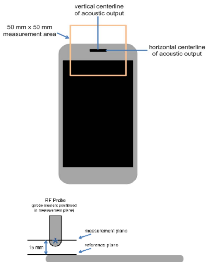
Fig 4.2 WD measurement and reference planes for RF emission measurements
