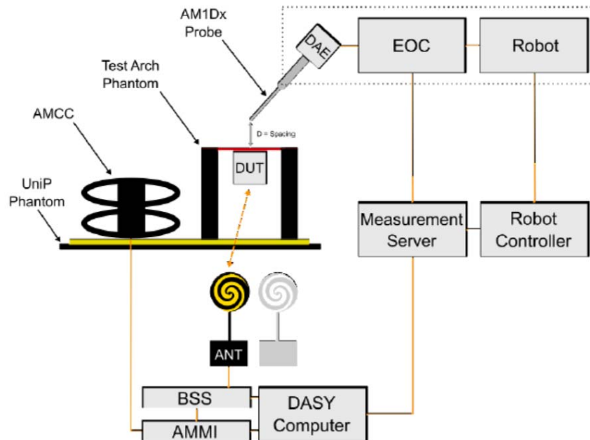
Fig 4.1 SPEAG T-Coil System Configurations
