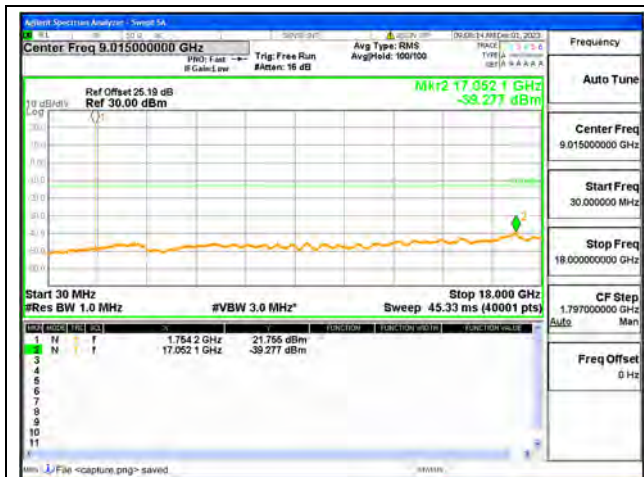
B4 / 1.4MHz / High CH / QPSK
