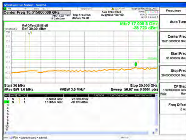
B7-30M-20G / 5MHz / Low CH / QPSK
