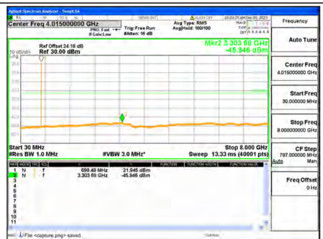
B12 / 3MHz / Low CH / QPSK
