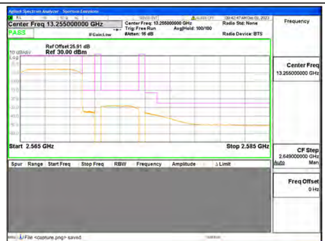
B7 / 5MHz / High CH / QPSK / FULL RB
