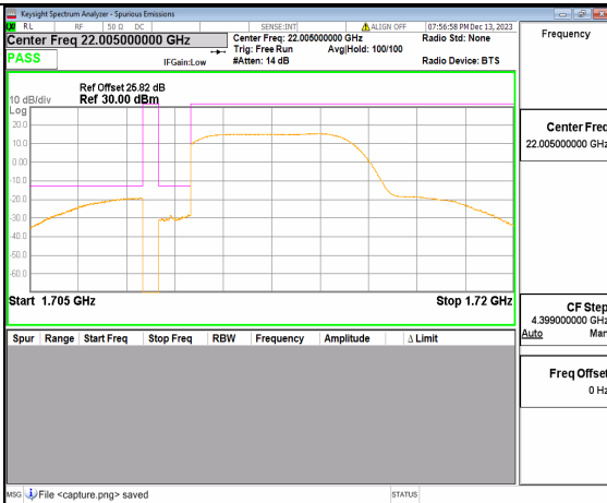
2A_n66 5M DFT-s-OFDM QPSK Outer_Full Low
