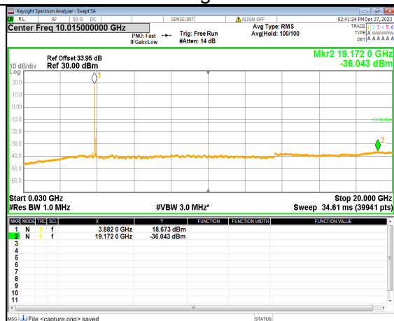
2A_n77(3700-3980MHz) (30MHz-20GHz) 100M DFT-s-OFDM QPSK Inner_1RB_Left
