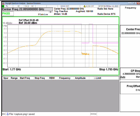
2A_n66 5M DFT-s-OFDM QPSK Outer_Full High
