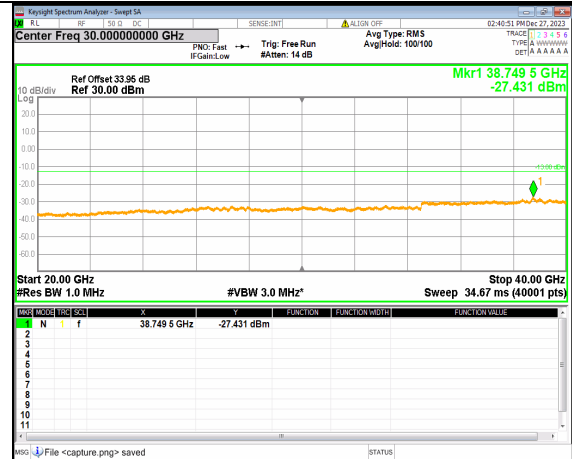
2A_n77(3700-3980MHz) (20GHz-40GHz) 100M DFT-s-OFDM BPSK Inner_1RB_Right High
