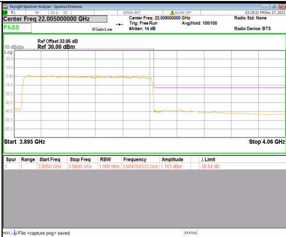
2A_n77(3700-3980MHz) 80M DFT-s-OFDM QPSK Outer_Full High
