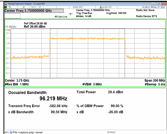
2A_n77(3700-3980MHz) 100M DFT-s-OFDM 64QAM Outer_Full Low
