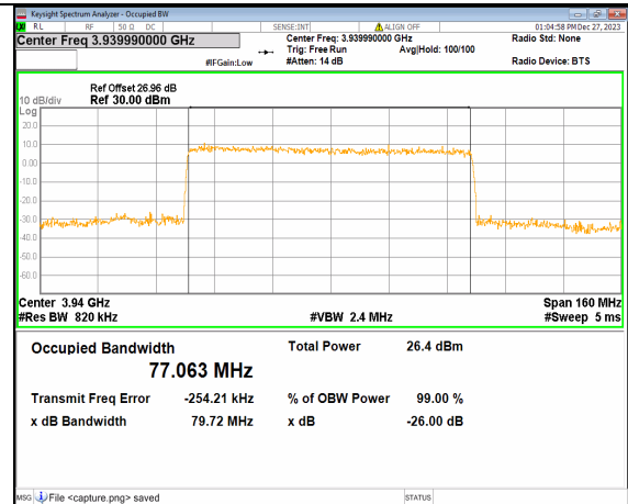
2A_n77(3700-3980MHz) 80M DFT-s-OFDM 64QAM Outer_Full High
