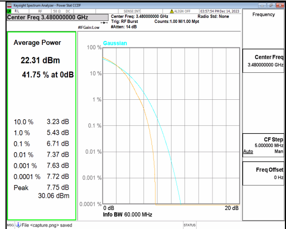
2A_n77(3450-3650MHz) 60M DFT-s-OFDM 256QAM Outer_Full Low
