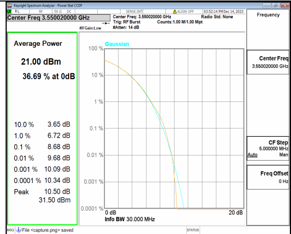
2A_n77(3450-3650MHz) 30M CP-OFDM 256QAM Outer_Full Mid
