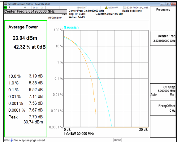
2A_n77(3450-3650MHz) 30M DFT-s-OFDM 256QAM Outer_Full High
