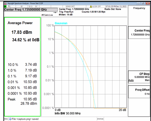
2A_n66 30M CP-OFDM 256QAM Outer_Full Low
