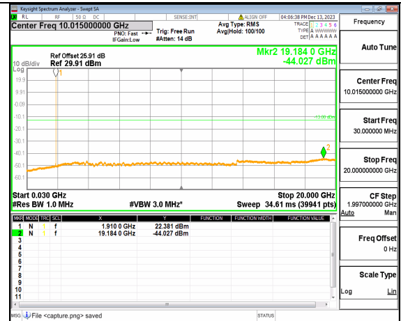
5A_n2 (30MHz-20GHz) 20M DFT-s-OFDM QPSK Inner_1RB_Right High
