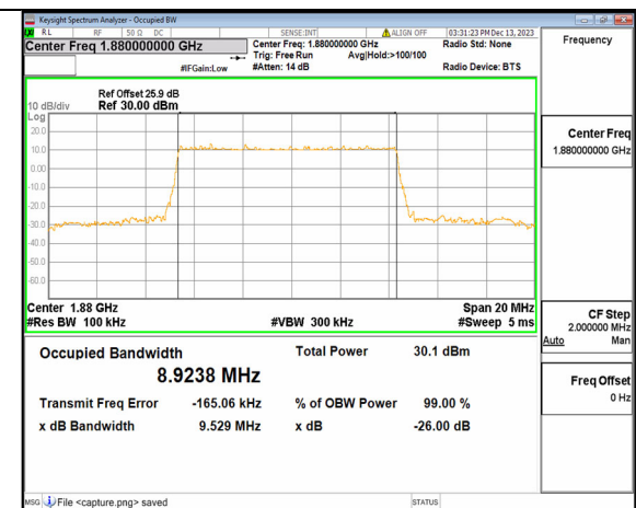
5A_n2 10M DFT-s-OFDM 64QAM Outer_Full Mid
