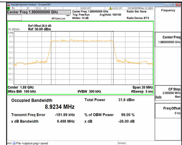
5A_n2 10M DFT-s-OFDM QPSK Outer_Full Mid
