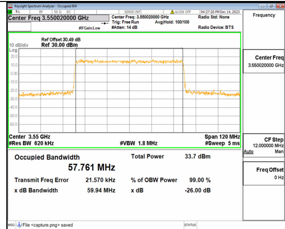
2A_n77(3450-3650MHz) 60M DFT-s-OFDM QPSK Outer_Full Mid
