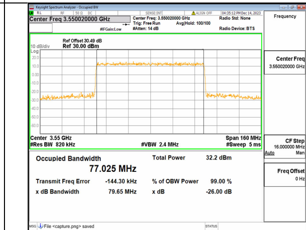
2A_n77(3450-3650MHz) 80M DFT-s-OFDM 64QAM Outer_Full Mid
