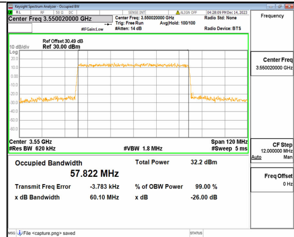
2A_n77(3450-3650MHz) 60M DFT-s-OFDM 64QAM Outer_Full Mid
