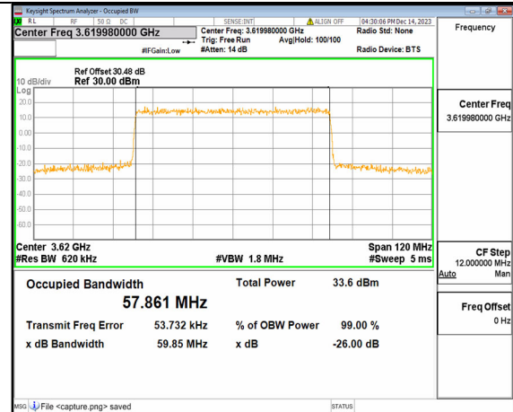
2A_n77(3450-3650MHz) 60M DFT-s-OFDM QPSK Outer_Full High
