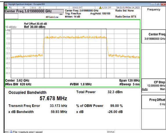
2A_n77(3450-3650MHz) 60M DFT-s-OFDM 64QAM Outer_Full High
