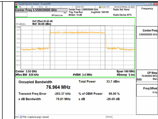
2A_n77(3450-3650MHz) 80M DFT-s-OFDM QPSK Outer_Full Mid
