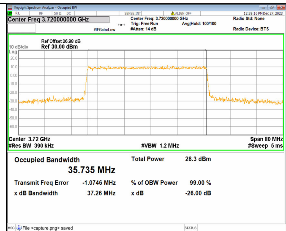
2A_n77(3700-3980MHz) 40M DFT-s-OFDM 64QAM Outer_Full Low
