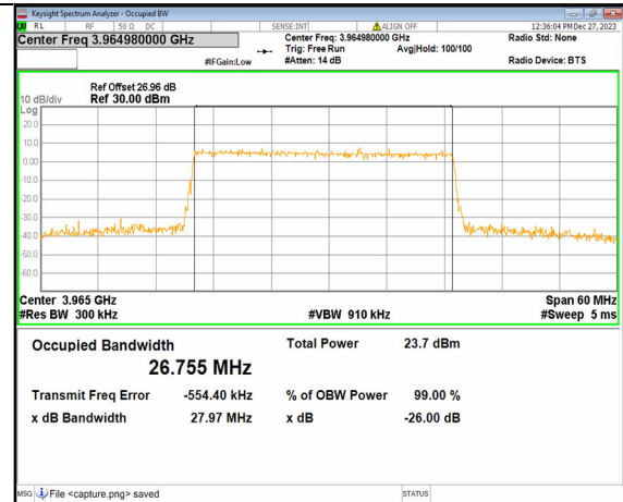
2A_n77(3700-3980MHz) 30M DFT-s-OFDM 64QAM Outer_Full High
