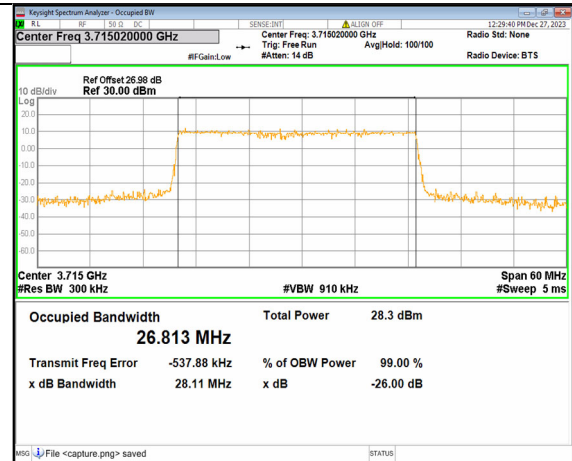
2A_n77(3700-3980MHz) 30M DFT-s-OFDM 64QAM Outer_Full Low
