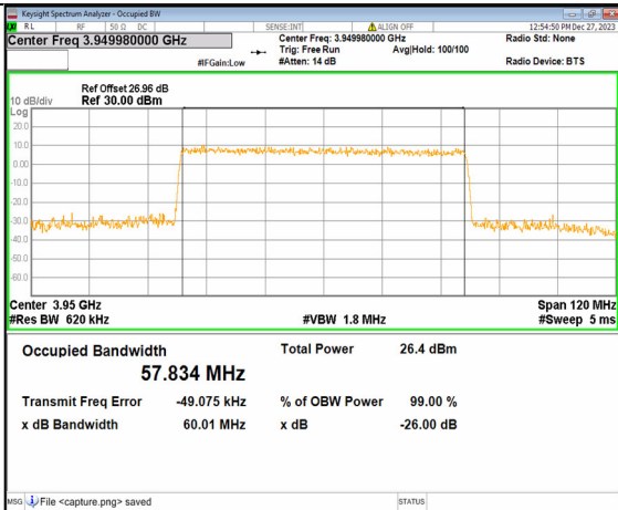
2A_n77(3700-3980MHz) 60M DFT-s-OFDM 16QAM Outer_Full High
