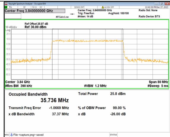
2A_n77(3700-3980MHz) 40M DFT-s-OFDM 64QAM Outer_Full Mid
