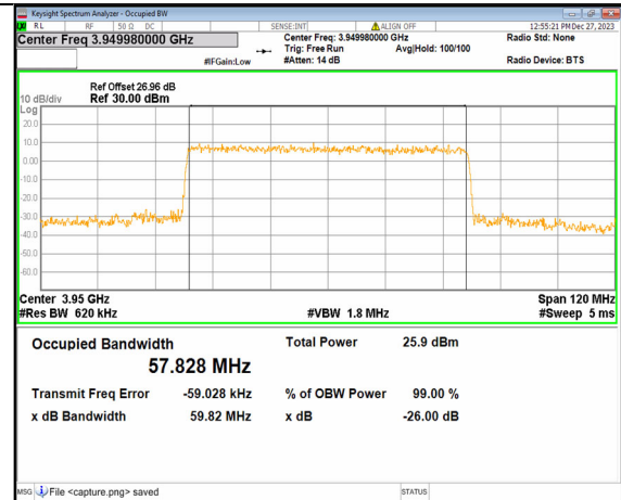
2A_n77(3700-3980MHz) 60M DFT-s-OFDM 64QAM Outer_Full High
