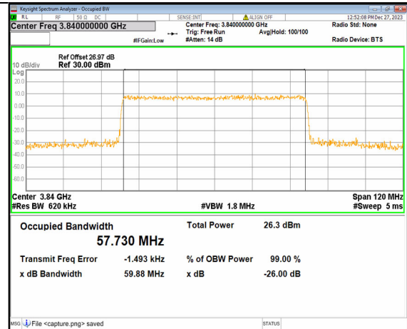
2A_n77(3700-3980MHz) 60M DFT-s-OFDM 64QAM Outer_Full Mid
