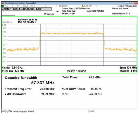
2A_n77(3700-3980MHz) 60M DFT-s-OFDM 16QAM Outer_Full Mid
