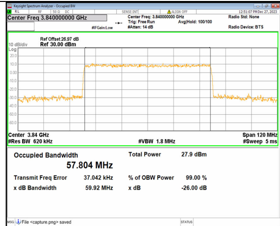
2A_n77(3700-3980MHz) 60M DFT-s-OFDM QPSK Outer_Full Mid
