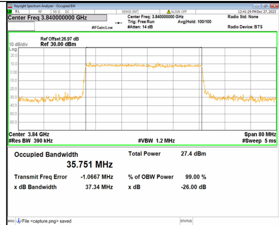
2A_n77(3700-3980MHz) 40M DFT-s-OFDM QPSK Outer_Full Mid
