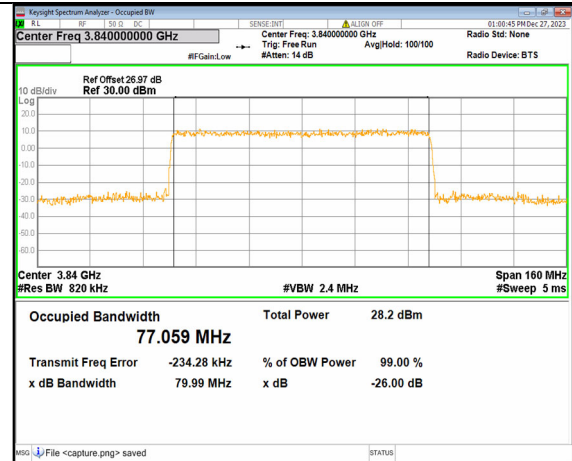
2A_n77(3700-3980MHz) 80M DFT-s-OFDM QPSK Outer_Full Mid
