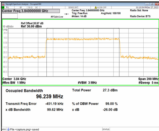
2A_n77(3700-3980MHz) 100M DFT-s-OFDM 16QAM Outer_Full Mid
