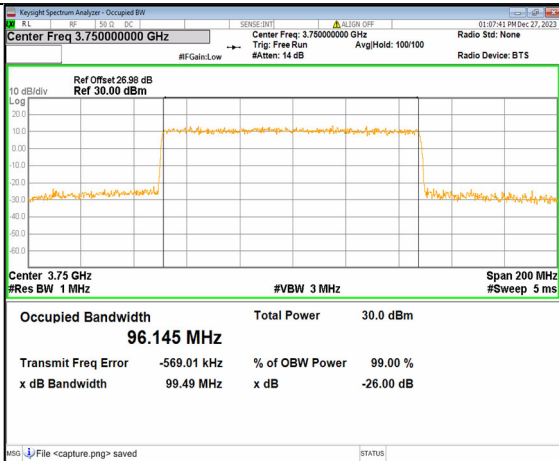
2A_n77(3700-3980MHz) 100M DFT-s-OFDM 16QAM Outer_Full Low
