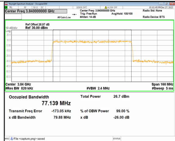
2A_n77(3700-3980MHz) 80M DFT-s-OFDM 64QAM Outer_Full Mid
