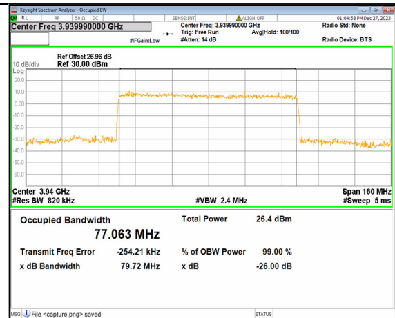
2A_n77(3700-3980MHz) 80M DFT-s-OFDM 64QAM Outer_Full High
