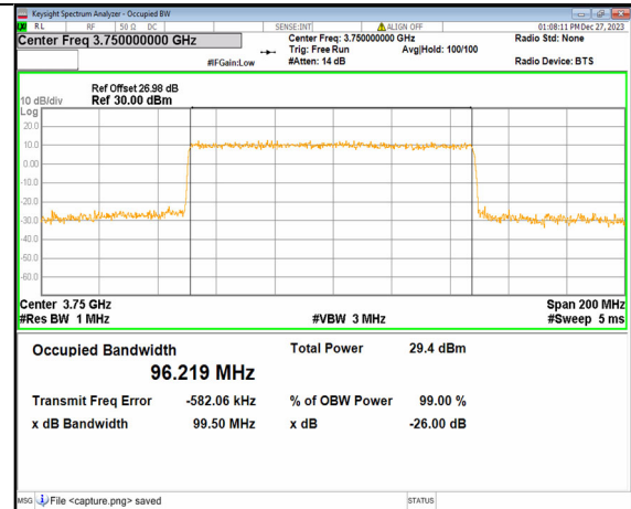
2A_n77(3700-3980MHz) 100M DFT-s-OFDM 64QAM Outer_Full Low
