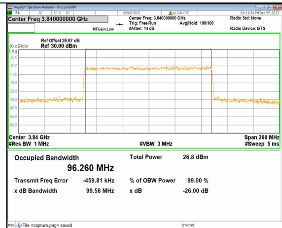
2A_n77(3700-3980MHz) 100M DFT-s-OFDM 64QAM Outer_Full Mid
