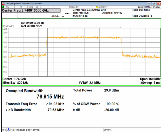
2A_n77(3700-3980MHz) 80M DFT-s-OFDM 16QAM Outer_Full Low
