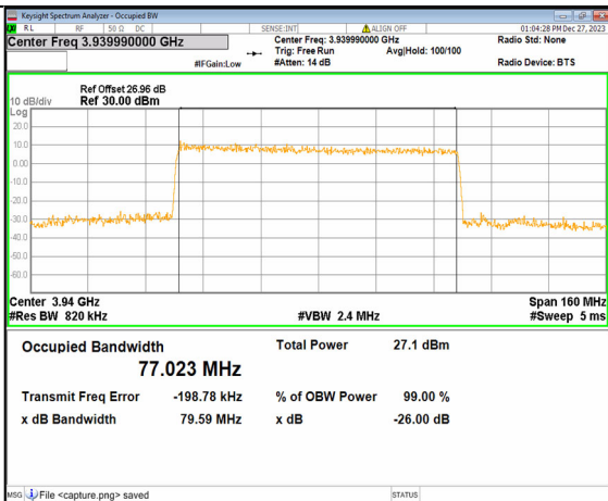
2A_n77(3700-3980MHz) 80M DFT-s-OFDM 16QAM Outer_Full High
