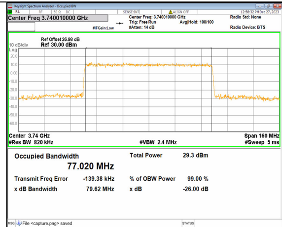
2A_n77(3700-3980MHz) 80M DFT-s-OFDM 64QAM Outer_Full Low
