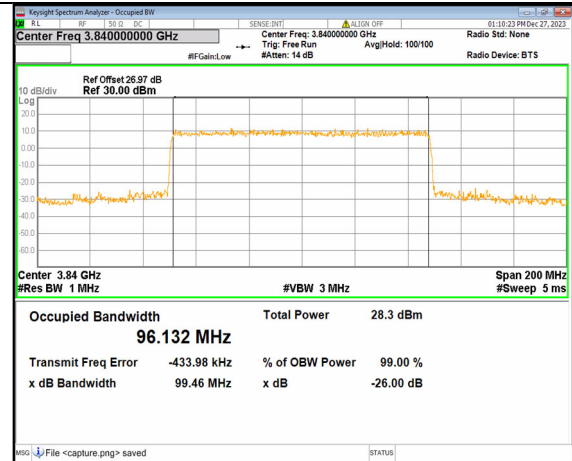
2A_n77(3700-3980MHz) 100M DFT-s-OFDM QPSK Outer_Full Mid
