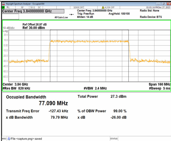
2A_n77(3700-3980MHz) 80M DFT-s-OFDM 16QAM Outer_Full Mid
