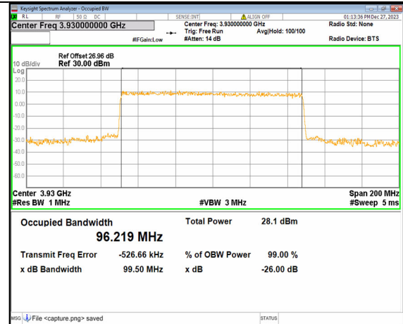
2A_n77(3700-3980MHz) 100M DFT-s-OFDM QPSK Outer_Full High
