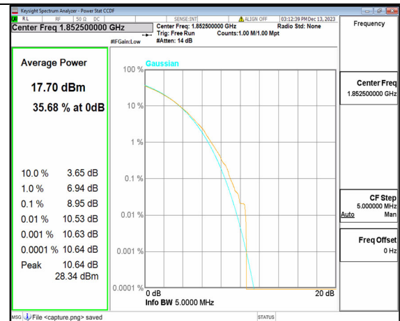
5A_n2 5M CP-OFDM 256QAM Outer_Full Low
