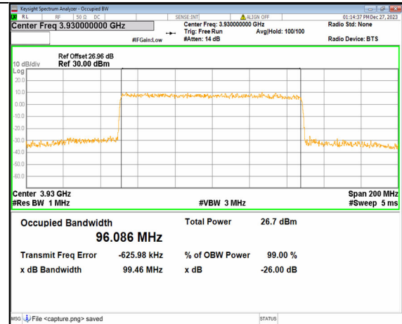
2A_n77(3700-3980MHz) 100M DFT-s-OFDM 64QAM Outer_Full High
