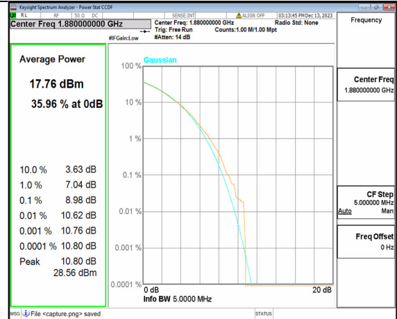
5A_n2 5M CP-OFDM 256QAM Outer_Full Mid
