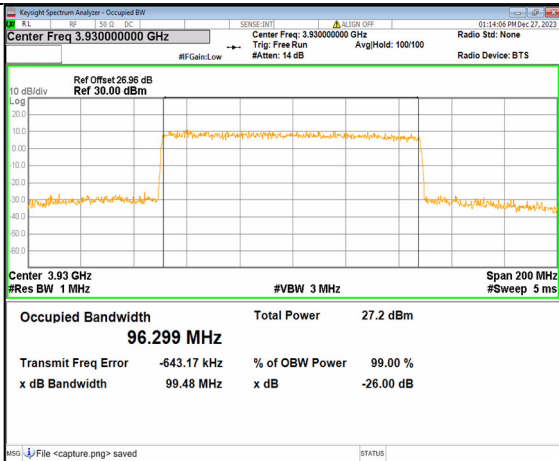
2A_n77(3700-3980MHz) 100M DFT-s-OFDM 16QAM Outer_Full High
