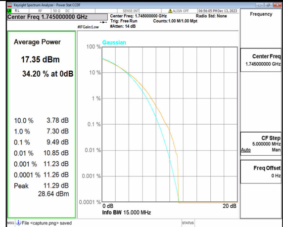
2A_n66 15M CP-OFDM 256QAM Outer_Full Mid
