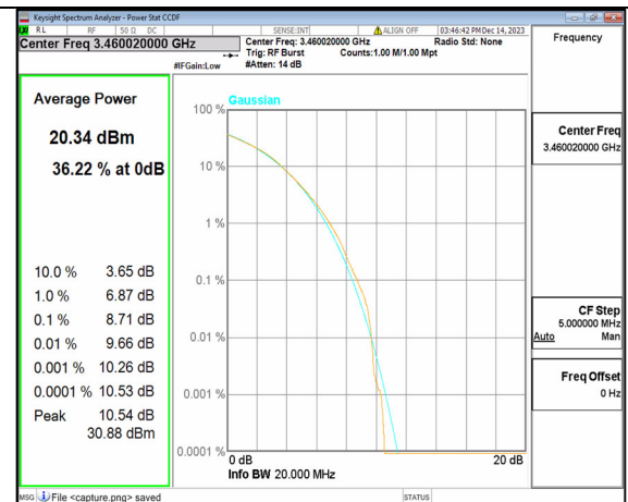
2A_n77(3450-3650MHz) 20M CP-OFDM 256QAM Outer_Full Low
