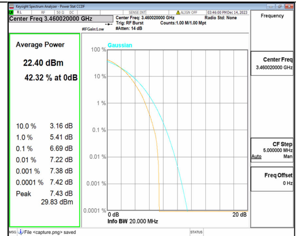
2A_n77(3450-3650MHz) 20M DFT-s-OFDM 256QAM Outer_Full Low
