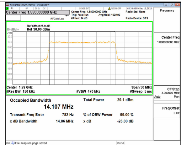
5A_n2 15M CP-OFDM QPSK Outer_Full Mid
