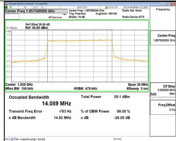
5A_n2 15M CP-OFDM QPSK Outer_Full Low
