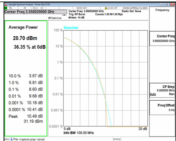
2A_n77(3450-3650MHz) 100M CP-OFDM 256QAM Outer_Full Mid
