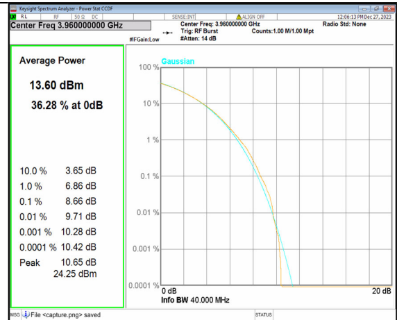
2A_n77(3700-3980MHz) 40M CP-OFDM 256QAM Outer_Full High
