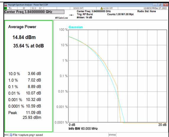
2A_n77(3700-3980MHz) 60M CP-OFDM 256QAM Outer_Full Mid
