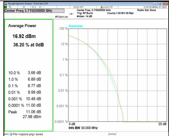
2A_n77(3700-3980MHz) 30M CP-OFDM 256QAM Outer_Full Low
