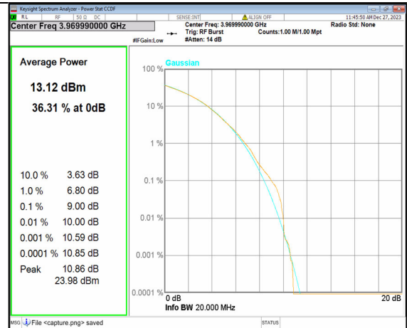
2A_n77(3700-3980MHz) 20M CP-OFDM 256QAM Outer_Full High
