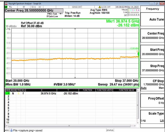
2A_n77(3450-3650MHz) (20GHz-37GHz) 60M DFT-s-OFDM QPSK Inner_1RB_Right Mid
