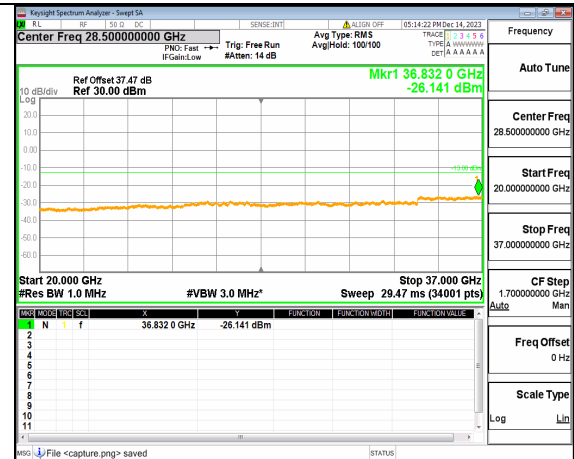
2A_n77(3450-3650MHz) (20GHz-37GHz) 30M DFT-s-OFDM QPSK Inner_1RB_Left High
