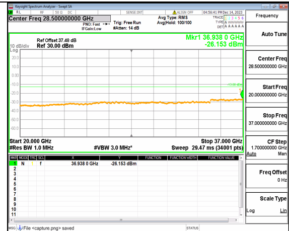
2A_n77(3450-3650MHz) (20GHz-37GHz) 20M DFT-s-OFDM QPSK Inner_1RB_Right Mid
