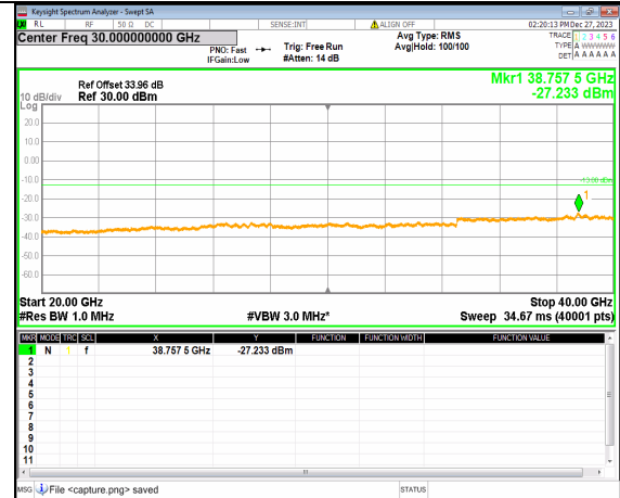
2A_n77(3700-3980MHz) (20GHz-40GHz) 80M DFT-s-OFDM BPSK Inner_1RB_Left Mid
