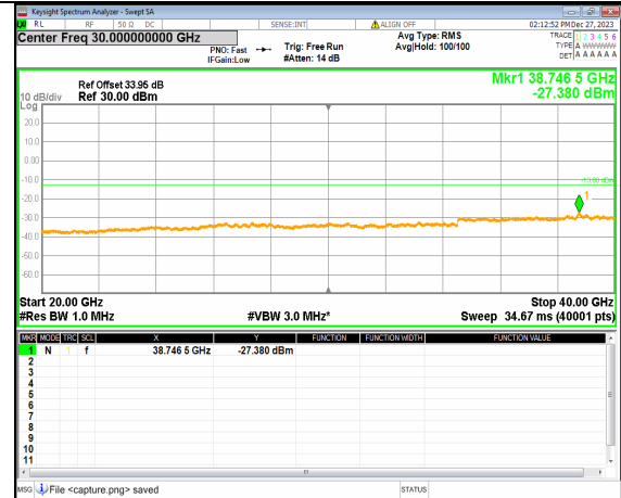
2A_n77(3700-3980MHz) (20GHz-40GHz) 60M DFT-s-OFDM QPSK Inner_1RB_Left High
