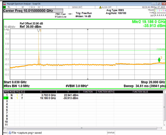
2A_n77(3700-3980MHz) (30MHz-20GHz) 100M DFT-s-OFDM QPSK Inner_1RB_Left Low
