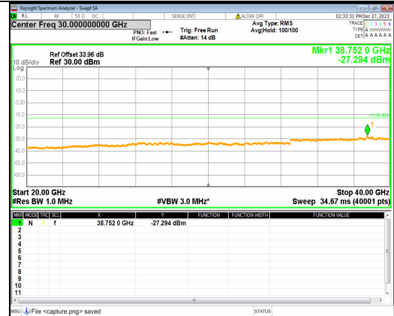
2A_n77(3700-3980MHz) (20GHz-40GHz) 100M DFT-s-OFDM QPSK Inner_1RB_Right Low
