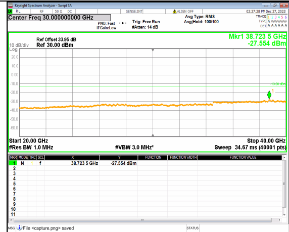
2A_n77(3700-3980MHz) (20GHz-40GHz) 80M DFT-s-OFDM QPSK Inner_1RB_Left High
