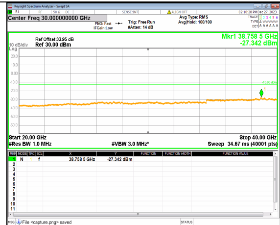
2A_n77(3700-3980MHz) (20GHz-40GHz) 60M DFT-s-OFDM BPSK Inner_1RB_Left High
