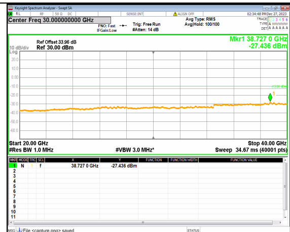
2A_n77(3700-3980MHz) (20GHz-40GHz) 100M DFT-s-OFDM BPSK Inner_1RB_Left Mid
