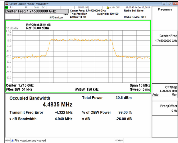
2A_n66 5M DFT-s-OFDM QPSK Outer_Full Mid
