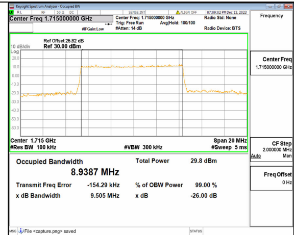
2A_n66 10M DFT-s-OFDM 64QAM Outer_Full Low
