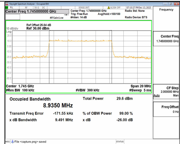
2A_n66 10M DFT-s-OFDM 64QAM Outer_Full Mid
