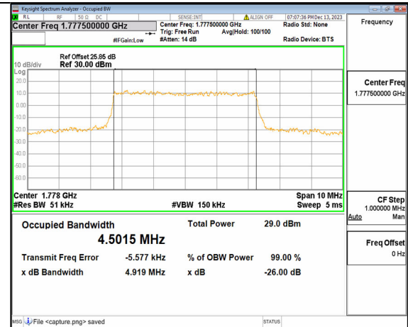
2A_n66 5M DFT-s-OFDM 64QAM Outer_Full High
