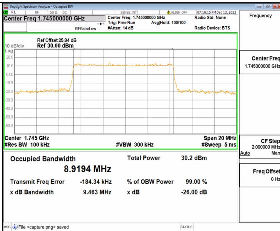
2A_n66 10M DFT-s-OFDM 16QAM Outer_Full Mid
