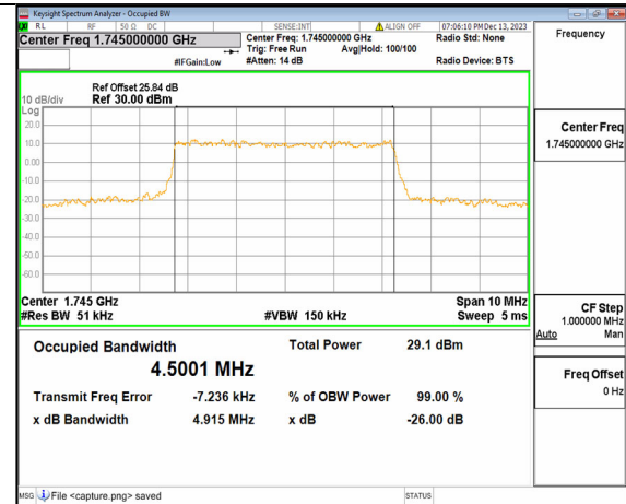
2A_n66 5M DFT-s-OFDM 64QAM Outer_Full Mid
