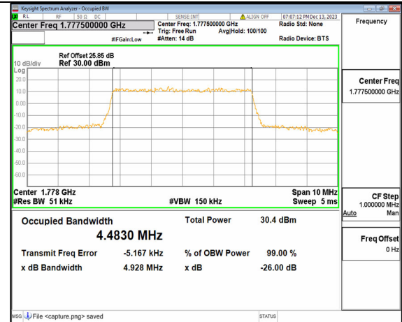
2A_n66 5M DFT-s-OFDM QPSK Outer_Full High
