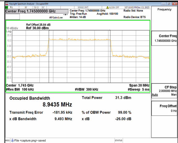
2A_n66 10M DFT-s-OFDM QPSK Outer_Full Mid
