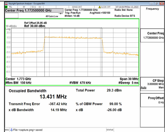
2A_n66 15M DFT-s-OFDM 64QAM Outer_Full High
