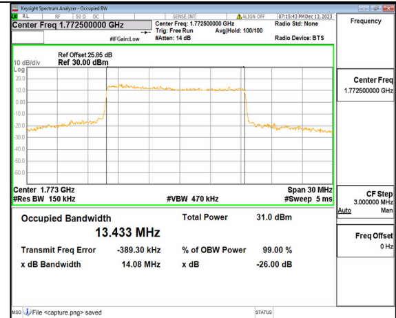
2A_n66 15M DFT-s-OFDM QPSK Outer_Full High
