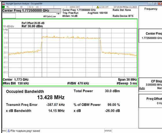
2A_n66 15M DFT-s-OFDM 16QAM Outer_Full High
