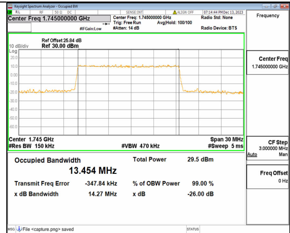
2A_n66 15M DFT-s-OFDM 64QAM Outer_Full Mid
