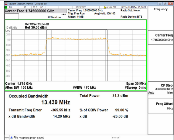
2A_n66 15M DFT-s-OFDM QPSK Outer_Full Mid
