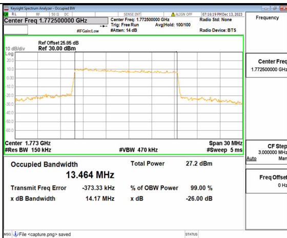
2A_n66 15M DFT-s-OFDM 256QAM Outer_Full High
