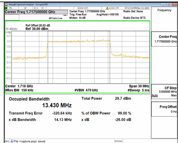
2A_n66 15M DFT-s-OFDM 64QAM Outer_Full Low
