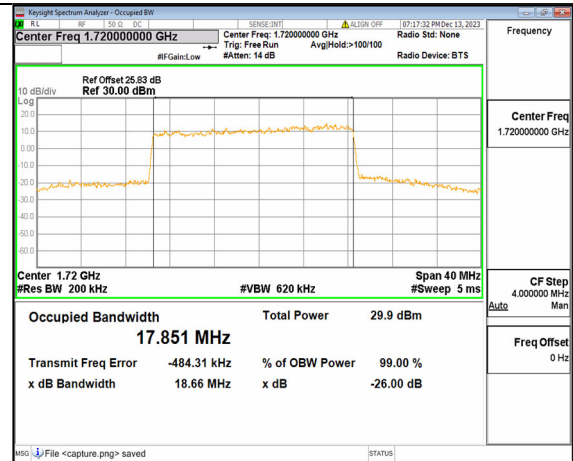
2A_n66 20M DFT-s-OFDM 64QAM Outer_Full Low
