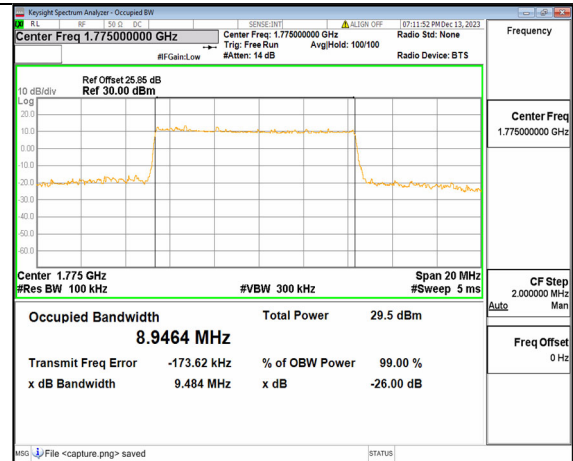
2A_n66 10M DFT-s-OFDM 64QAM Outer_Full High
