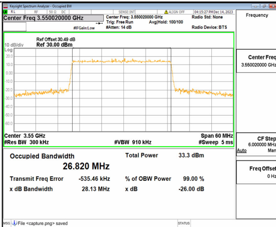
2A_n77(3450-3650MHz) 30M DFT-s-OFDM 16QAM Outer_Full Mid
