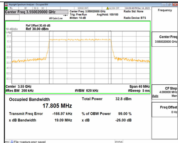
2A_n77(3450-3650MHz) 20M DFT-s-OFDM 64QAM Outer_Full Mid
