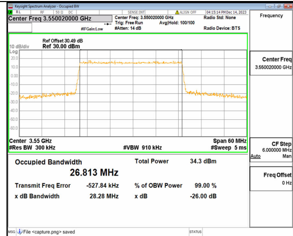
2A_n77(3450-3650MHz) 30M DFT-s-OFDM QPSK Outer_Full Mid
