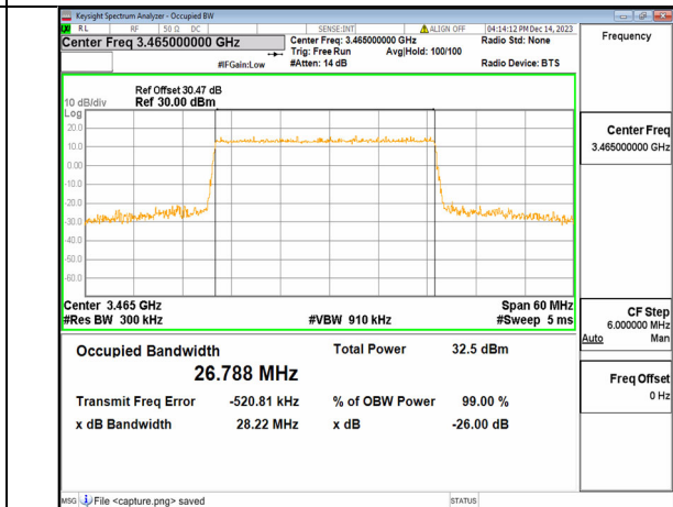
2A_n77(3450-3650MHz) 30M DFT-s-OFDM 64QAM Outer_Full Low
