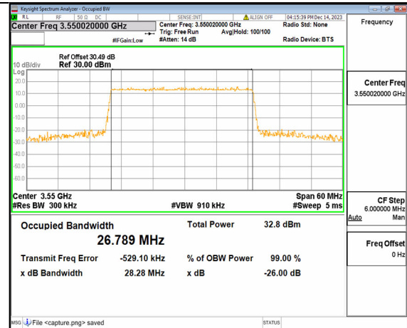
2A_n77(3450-3650MHz) 30M DFT-s-OFDM 64QAM Outer_Full Mid
