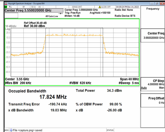
2A_n77(3450-3650MHz) 20M DFT-s-OFDM QPSK Outer_Full Mid
