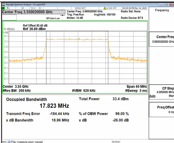
2A_n77(3450-3650MHz) 20M DFT-s-OFDM 16QAM Outer_Full Mid
