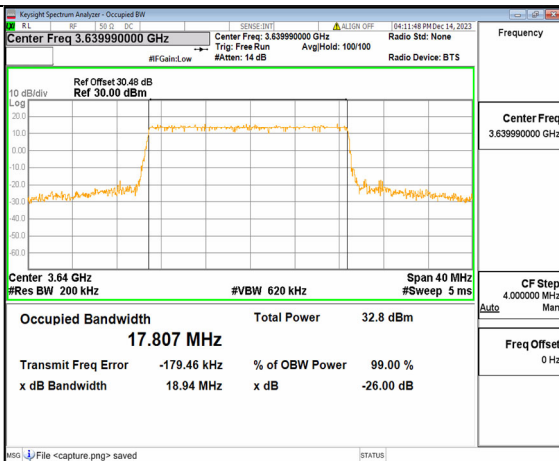
2A_n77(3450-3650MHz) 20M DFT-s-OFDM 16QAM Outer_Full High
