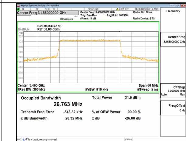
2A_n77(3450-3650MHz) 30M CP-OFDM QPSK Outer_Full Low
