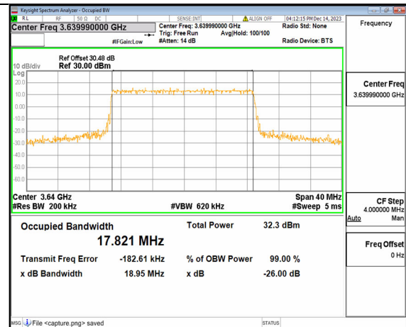
2A_n77(3450-3650MHz) 20M DFT-s-OFDM 64QAM Outer_Full High
